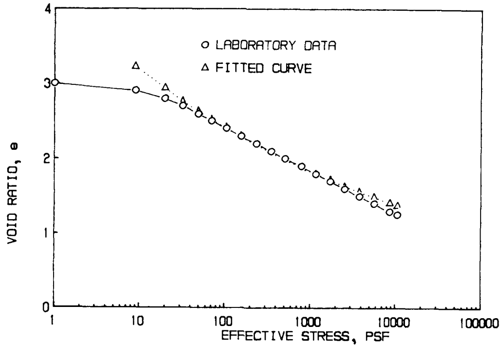
Figure 6. Void ratio-effective stress relationship for the Craney Island foundation soil
