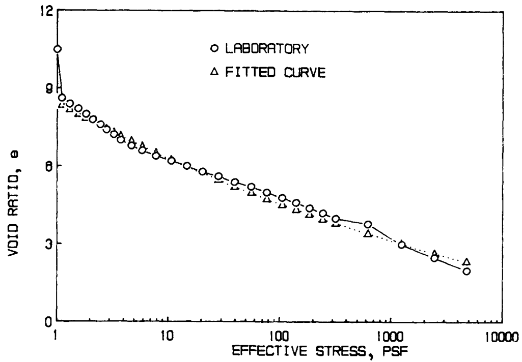
Figure 4. Void ratio-effective stress relationship for the Craney Island dredged material
