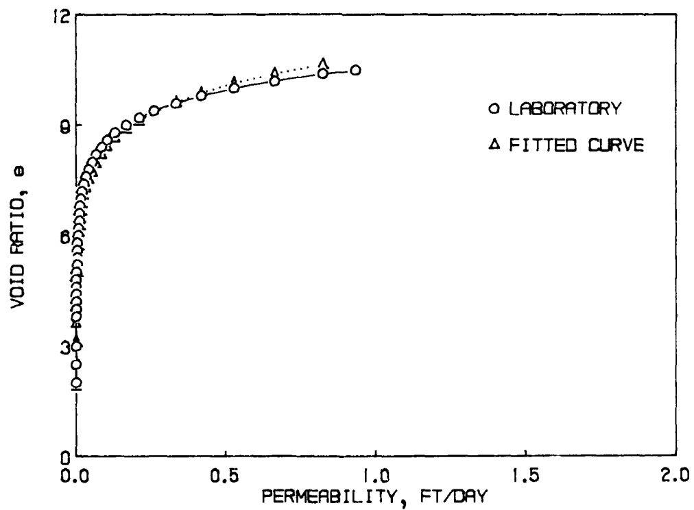
Figure 5. Void ratio-permeability relationship for the Craney Island dredged material
