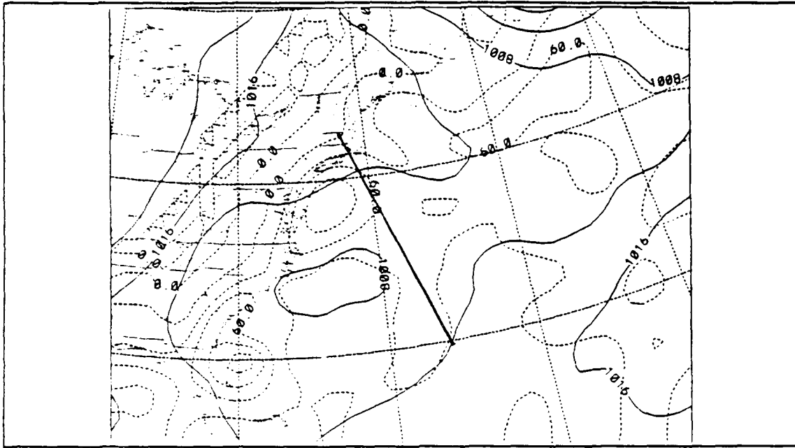
Figure 17. 0000 UTC 25 February 1986 Surface heat flux: in W/m^2 . Solid lines are sea-level pressure in mb.
