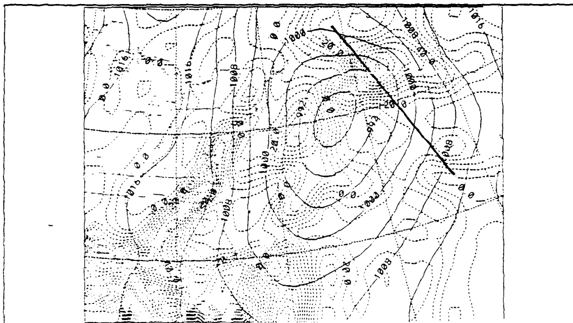
Figure 22. 0000 UTC 26 February 1986 Total increase in \theta ; Same as Fig. 14
