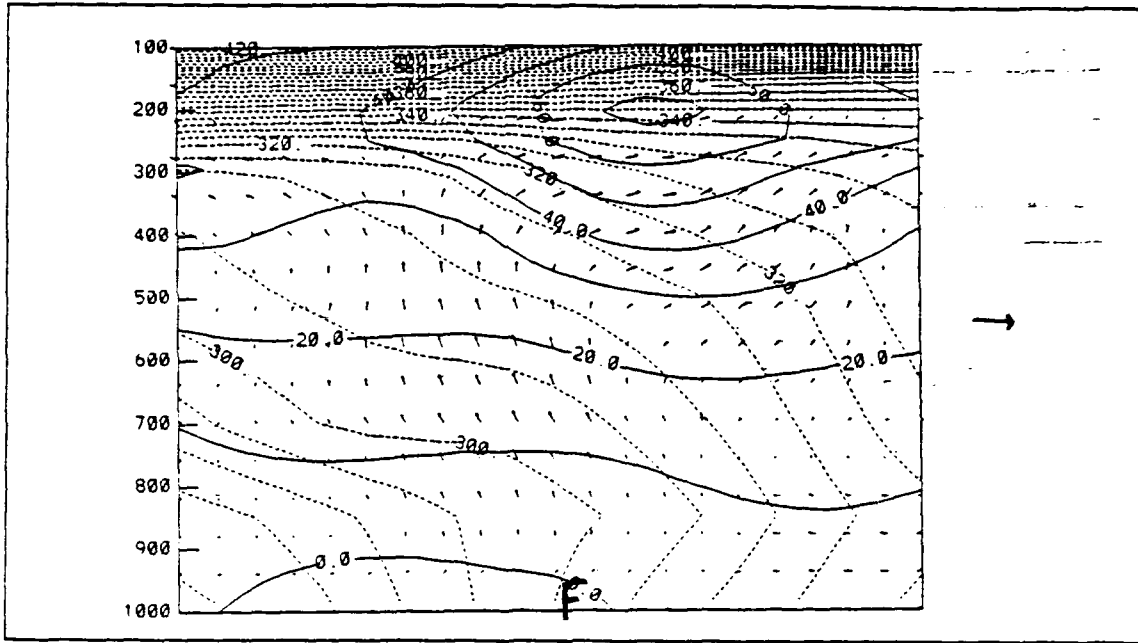
Figure 26. 0000 UTC 25 February 1986 Cross section of isotachs and \theta : Isotachs in m s (solid) and \theta , in K (dashed). Arrows are ageostrophic flow, with maximum vector to right of figure 20-m s. Surface frontal location indicated by F. Location of cross section indicated in Fig. 3.
