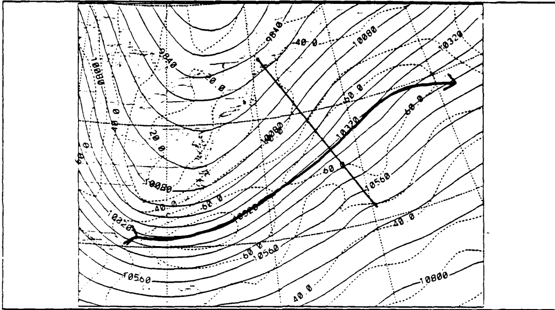
Figure 5. 1200 UTC 25 February 1986 Upper-Level Analysis: Same as Fig. 3
