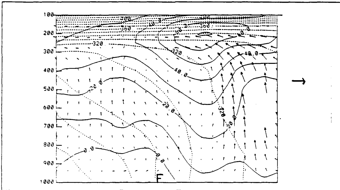
Figure 27. 1200 UTC 25 February 1986 Cross section of isotachs and \theta ; Same as Fig. 26 Location of cross section indicated in Fig. 5.
