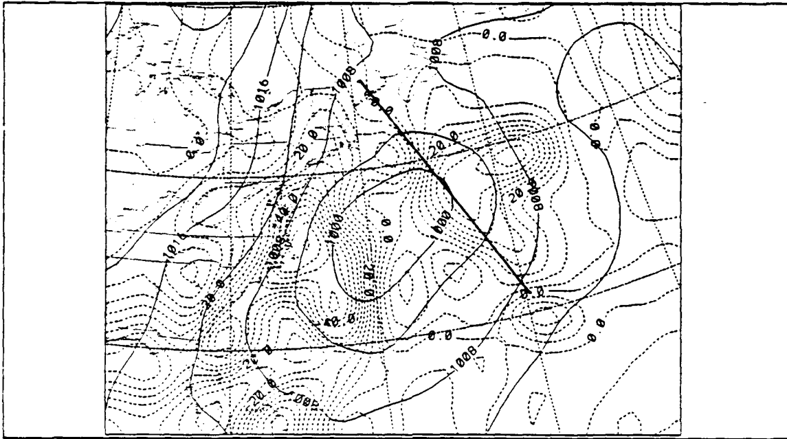
Figure 20. 1200 UTC 25 February 1986 Horizontal advection of \theta : Same as Fig. 15
