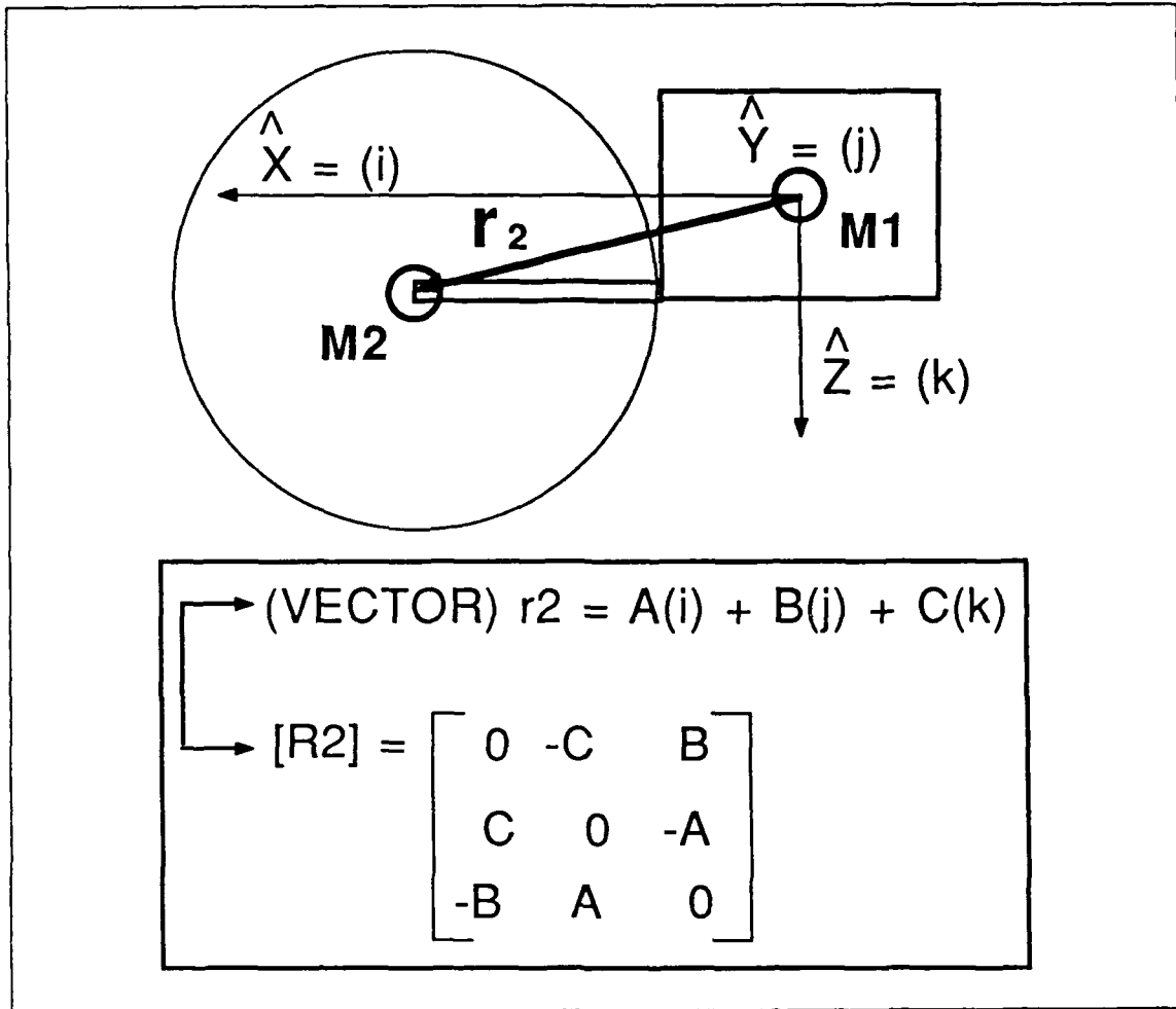
Figure 8. Skew-Symmetric Matrix
