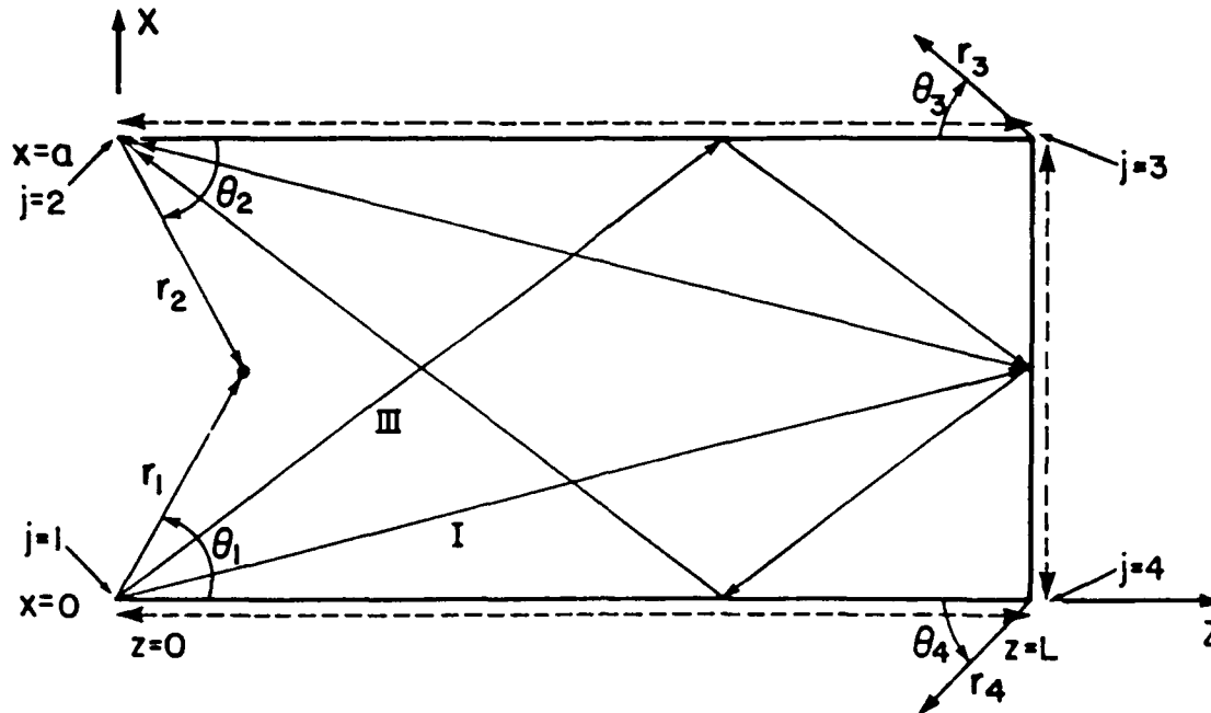
Fig. 4 Thin-walled rectangular trough of infinite length along y. Relevant internal and external ray interactions are schematized by solid and dashed lines, respectively, with the interior Roman numerals identifying the number of (internal) reflections between diffraction events at the edges j=1,2 . The sketch includes up to three internal reflections. Local coordinates (r_j, \theta_j) identify phenomena associated with edge j .
