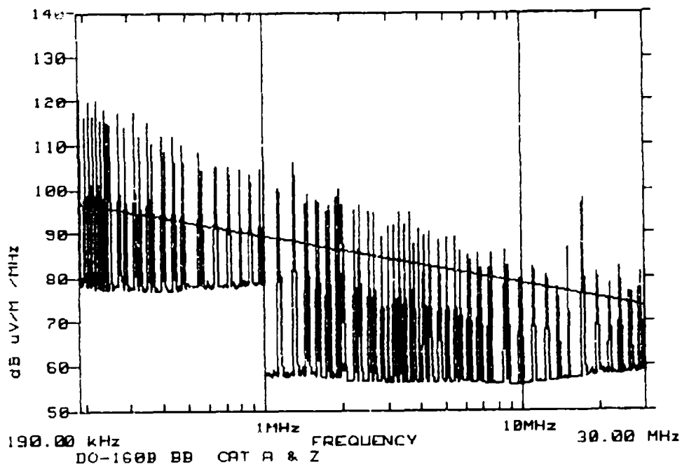
Figure A-8 Electric field emissions from the composite wing in a vertical orientation as per DO160B. The frequency range is 190 kHz to 30 MHz. Shielding has been placed over the power supplies. Emission levels exceed standards.
