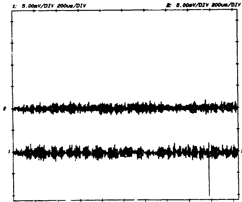
Figure B-7 Trace 1 is the induced voltage on a shielded coaxial cable terminated into a 50\Omega resistor. Trace 2 is the induced voltage waveform for the telephone cable terminated into 50\Omega . Both cables are terminated by 50\Omega resistors. The induced voltage levels for both traces are below the noise threshold.
