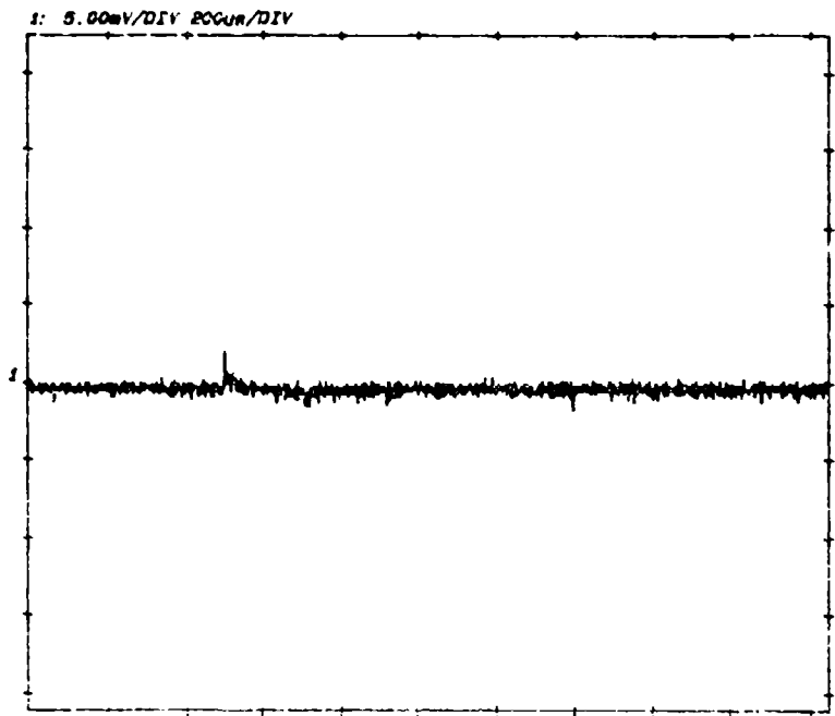
Figure B-3 Trace of induced voltage on an unshielded telephone cable run behind the module with both ends terminated by 50Ω resistors. The induced voltage is below 5mV.
