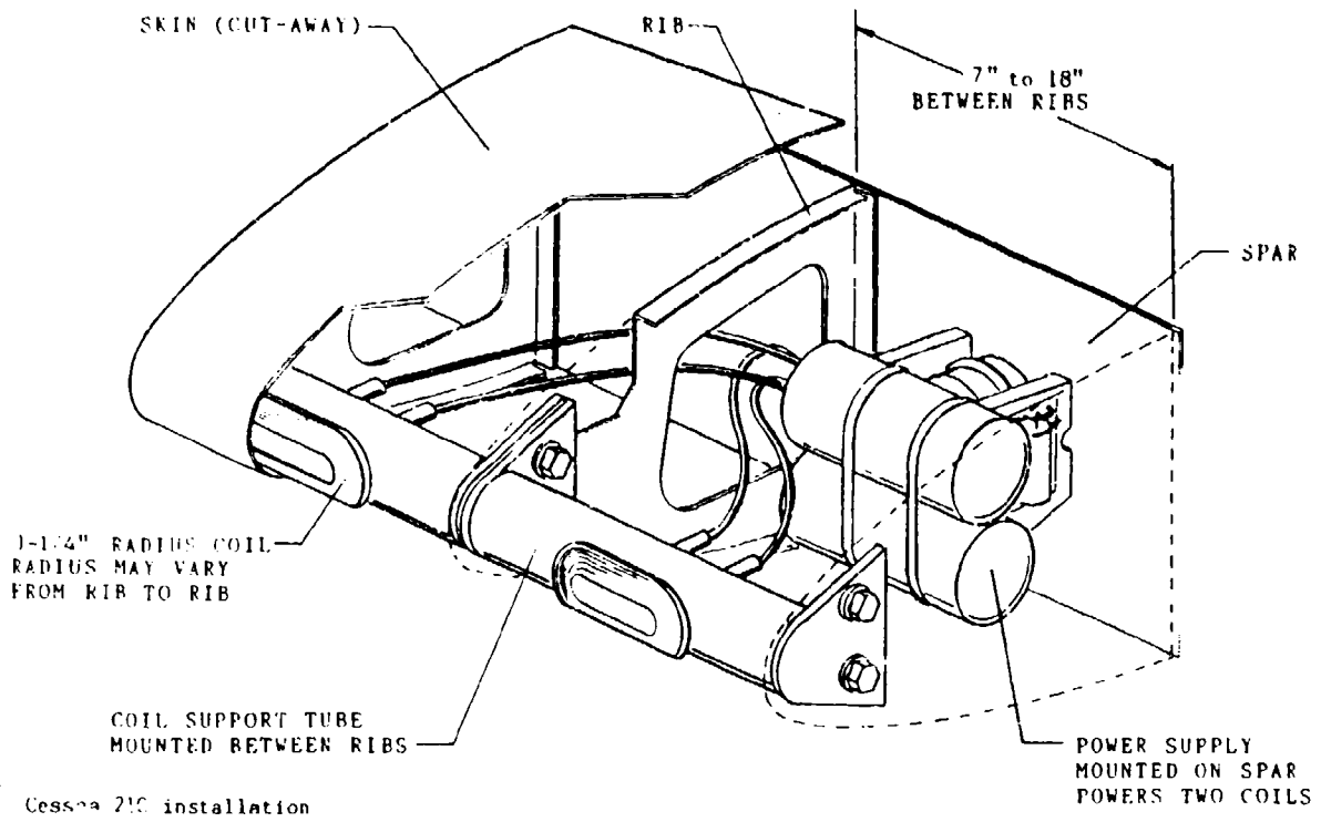
FIGURE 1 NOSE COILS INSTALLED IN THE ALUMINUM WING ON TUBULAR MOUNTS.
