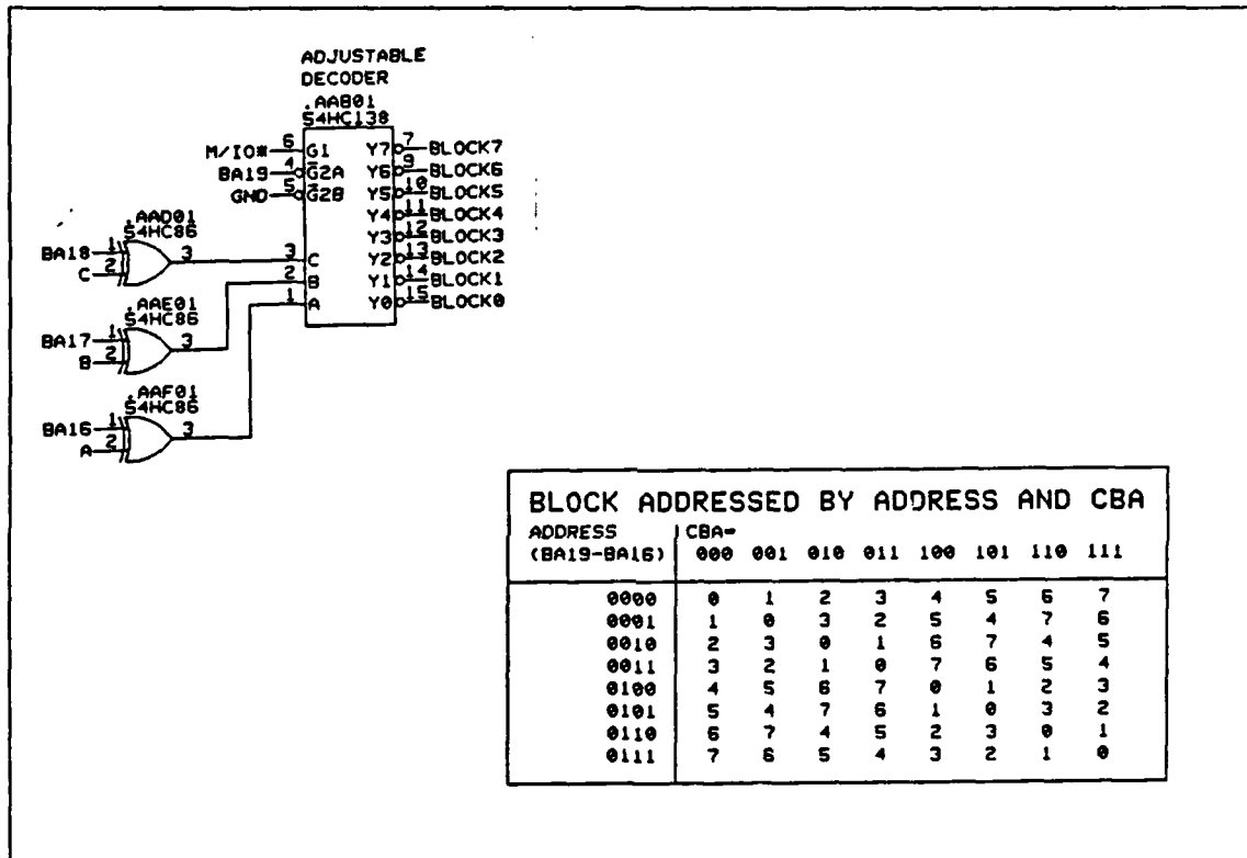
Figure 31. Dynamic memory decoding circuit and resulting mappings
