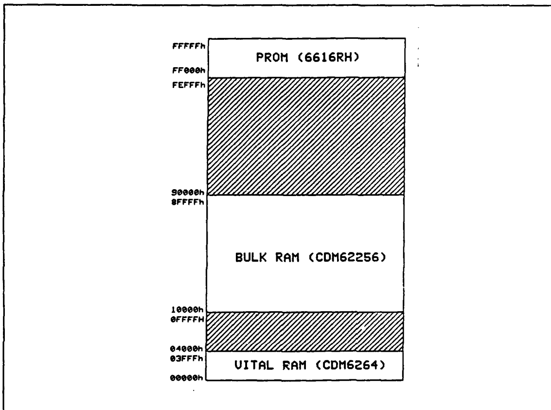
Figure 30. PANSAT memory address map
