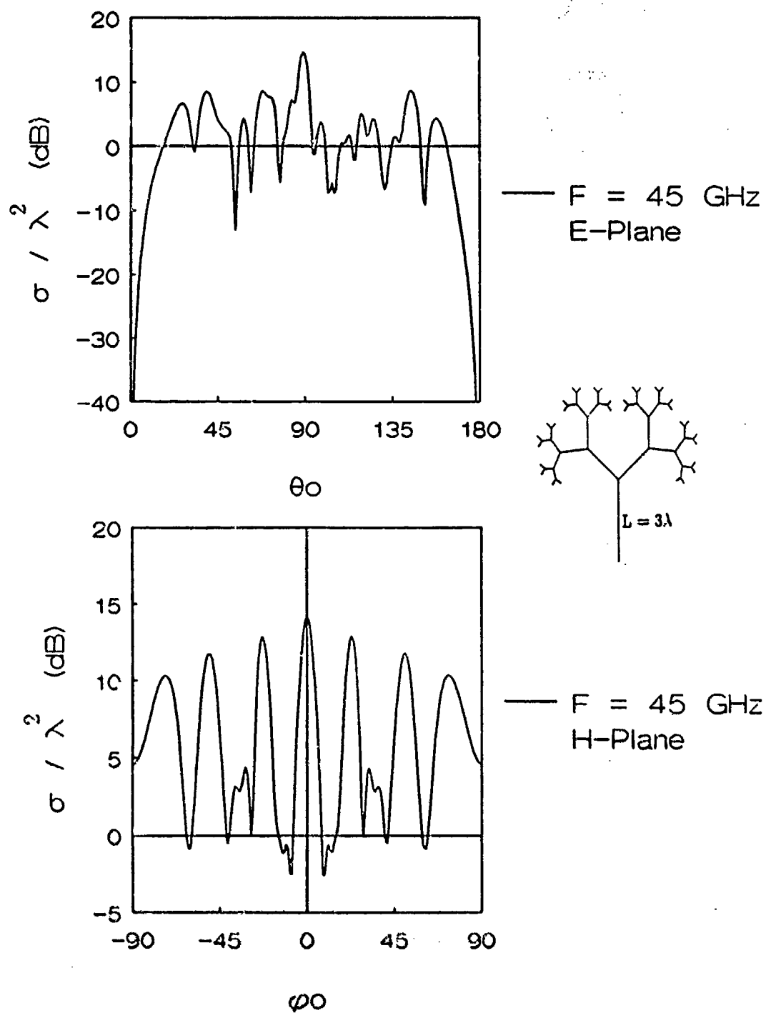
Figure 5.16 Normalized RCS at F = 45 GHz of a Planar Fractal Tree with r = 0.60 and \theta = 95.89^\circ .
