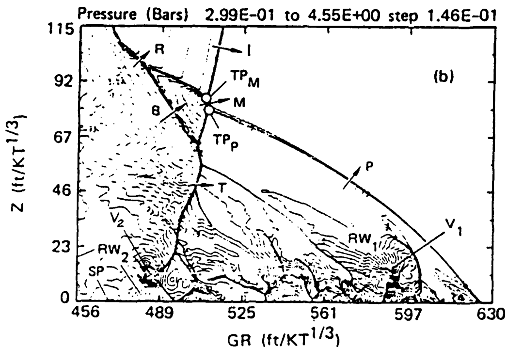
Figure 1. Density and pressure contours for a numerical calculation of a precursed blast wave.
