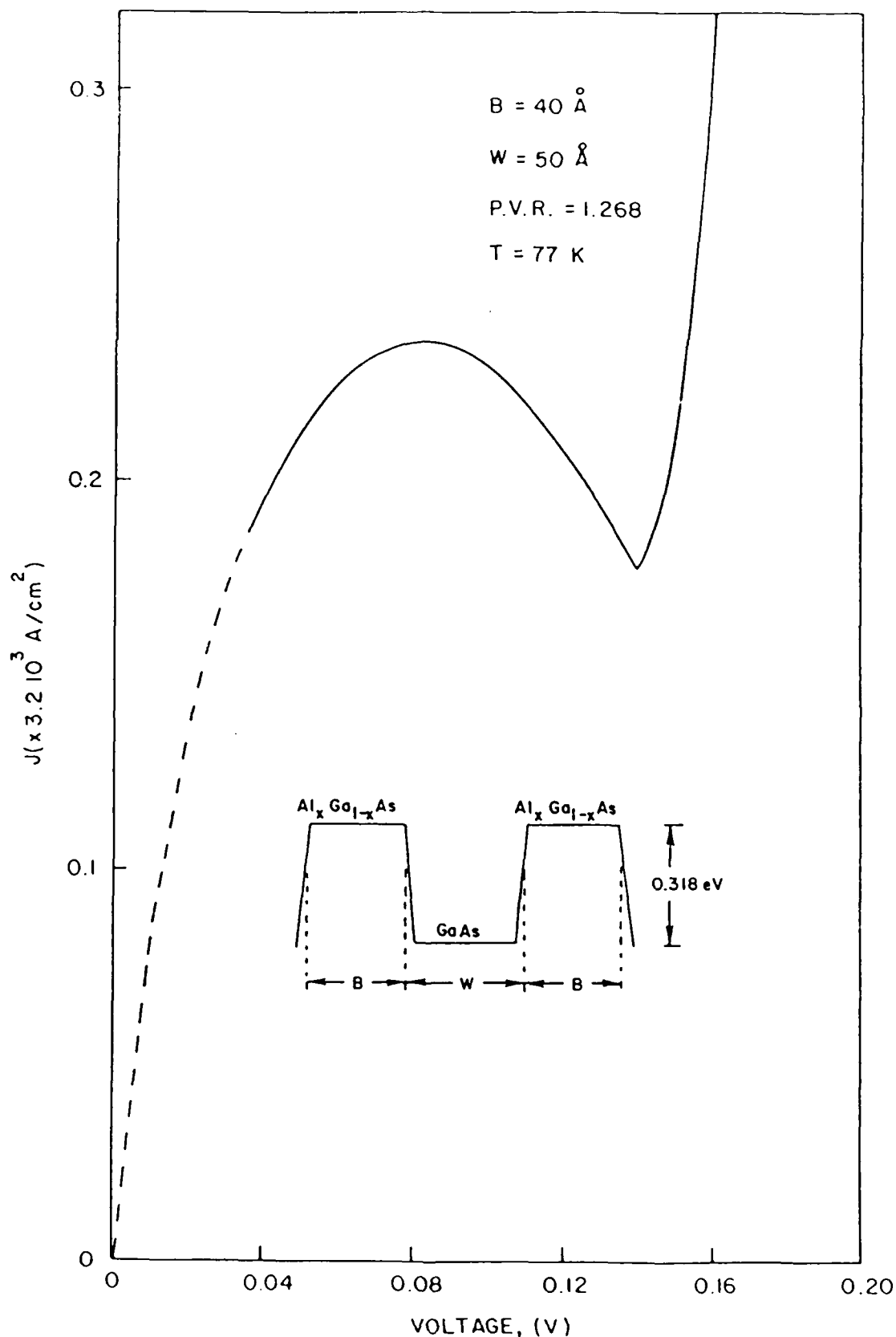
Figure 14: Current-voltage characteristic for RTD shown in the insert. The barrier height is 0.318eV and the effective mass is assumed to be constant ( m_{\text{GaAs}}^* = 0.067m_0 ). The doping profile of type II is considered in our numerical simulations. However, the 50Å regions on both sides of the RTD were assumed to be undoped. The dashed line is the expected shape of the I-V curve at low value of bias.
