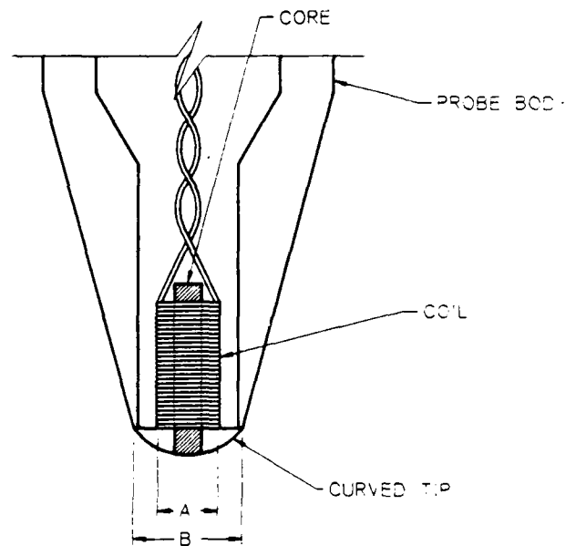
b. VIEW "X" NON-SHIELDED (TYPE N)
