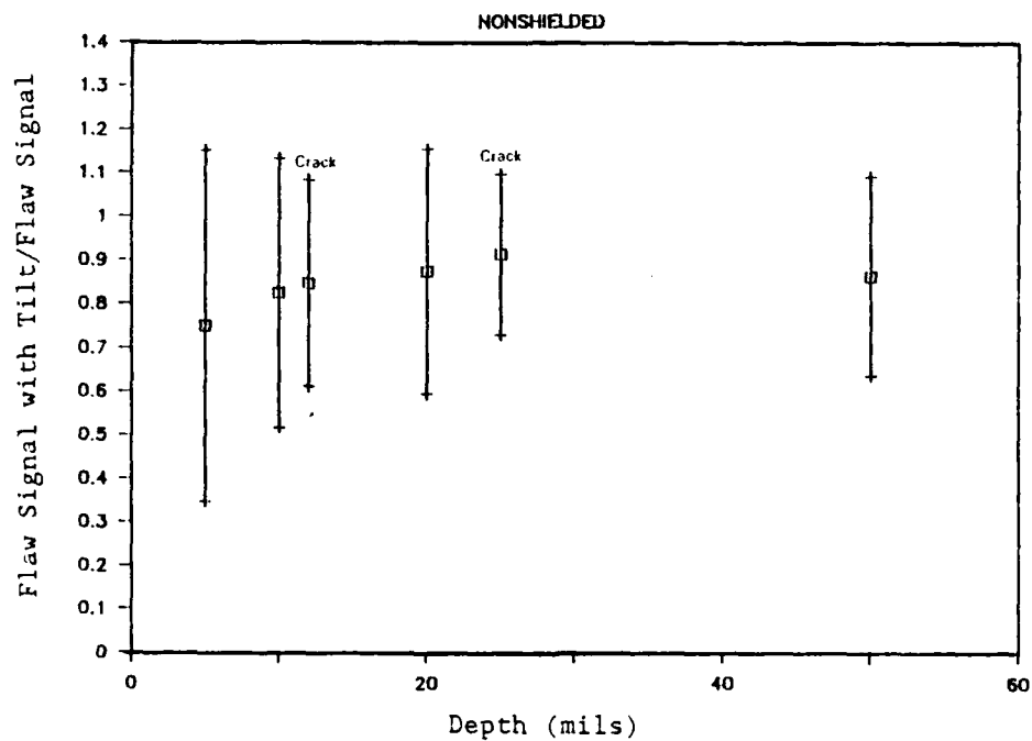
Figure 5-6. Effect of 10-degree probe tilt on flaw signal for probes tested. (Boxes represent mean value, and length of vertical lines are mean \pm two standard deviations).
