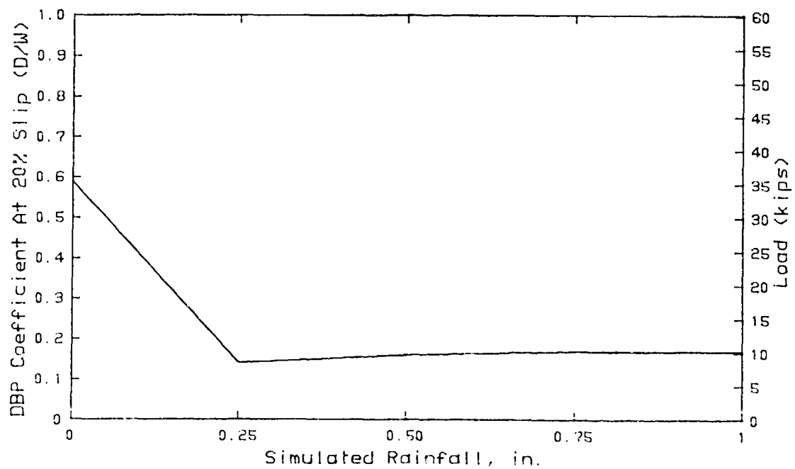
20%, Drawbar Pull Coefficient HEMTT; Duckport, La; CL Soil
