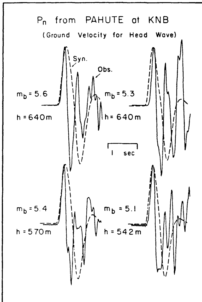
Figure 20. Observed versus synthetic waveforms at KNB for Pahute events. All assumptions are the same as in Figure 16.
