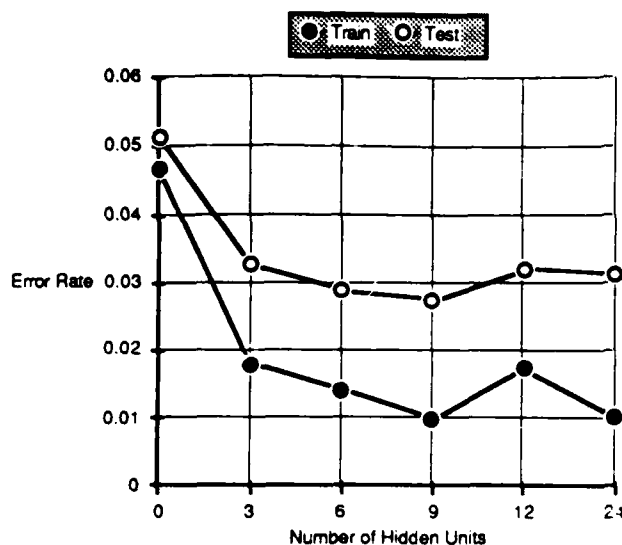
Figure 10: Neural Net Error Rates for Thyroid Data
