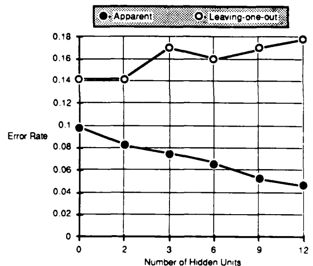
Figure 6: Neural Net Error Rates for Appendicitis Data
