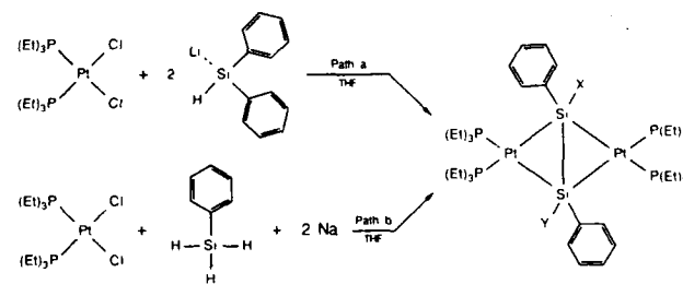
Scheme 1 a
