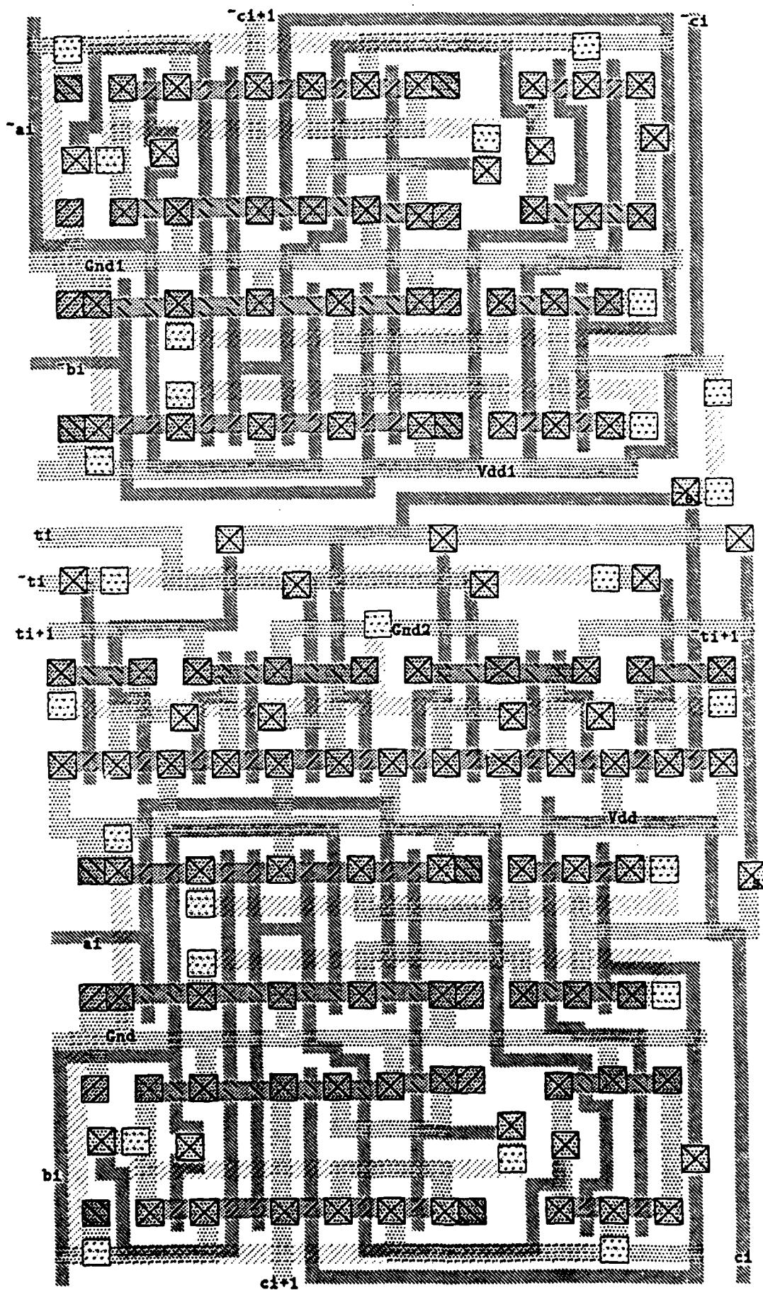
Fig. 14 Layout of Duplicated Adder Cell
