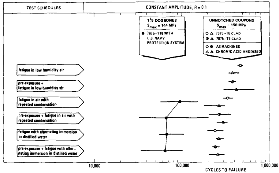
Fig. 3.4 SAAB fatigue life data contribution to the FACT programme
