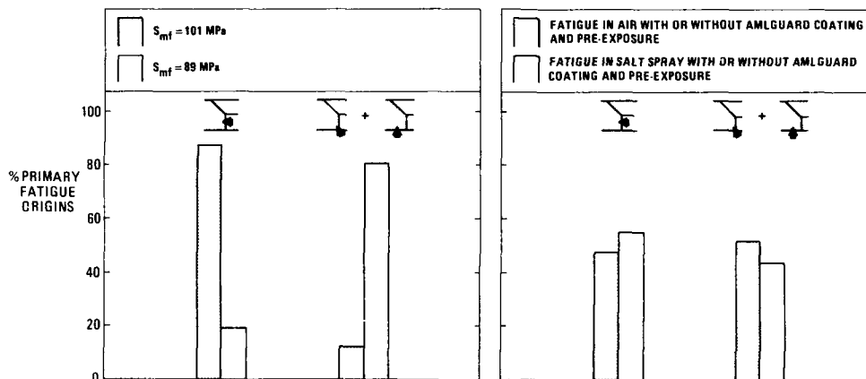
Fig. 7.7 Effects of stress and environment on locations of primary origins for monolithic 2024-T3 Alclad specimens tested as part of the NLR and LRTH MINITWIST fatigue contribution to FACT
