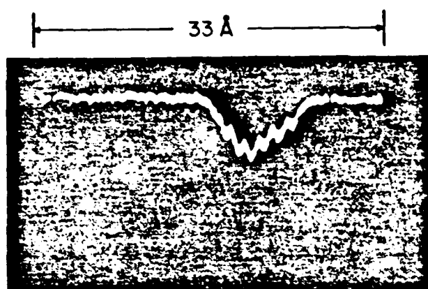
Fig. 5. Spectrum of pulses of 7 ps pulsewidth. FWHM \approx 5.5 Å. The spectrometer has a resolution of 0.156 Å/diode at 1 \mu\text{m} .
