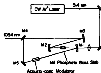
Fig. 1. Schematic of the CW actively mode-locked Nd:phosphate glass laser oscillator. M1 is a dichroic-coated plano-concave mirror with R = 30 cm. M2 is an R = 30 cm plano-concave mirror with HR coating. M3 and M5 are plano mirrors with HR coating. M4 is a plano mirror with a reflectance of 97 percent.
