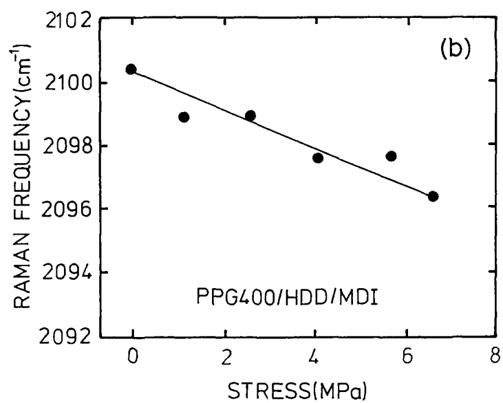
Figure 24. Variation of the position of the 2100\text{cm}^{-1} peak in PPG400/HDD/MDI with Deformation a) Dependence upon strain b) Dependence upon stress.
