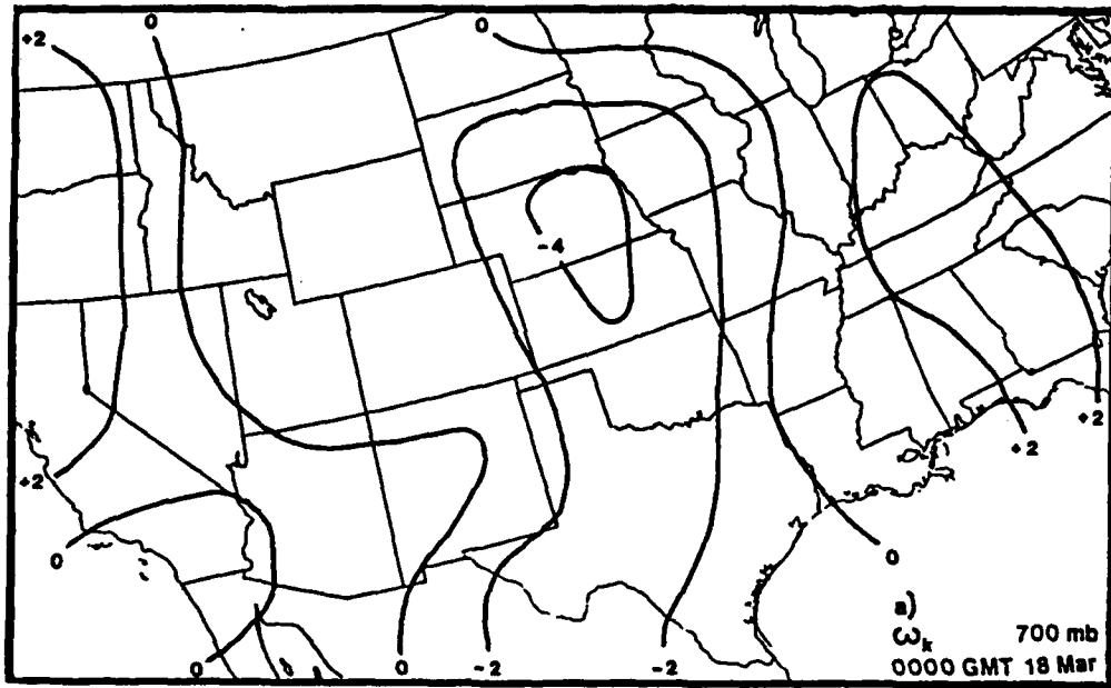
Fig. 7 As in Fig. 6, but for 0000 GMT 18 March 1986.
