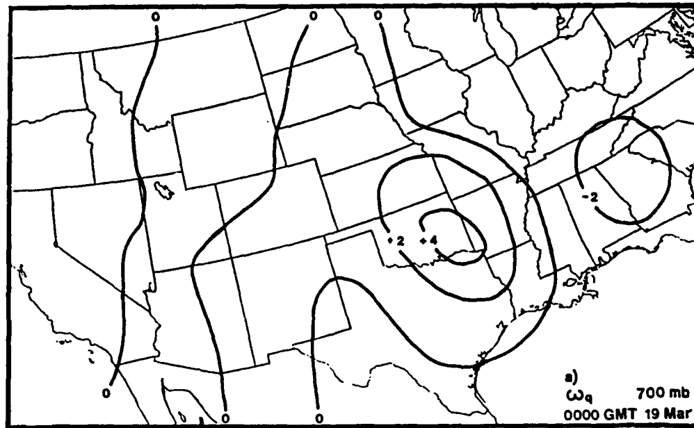
Fig. 26 As in Fig. 23, but for 0000 GMT 19 March 1986.
