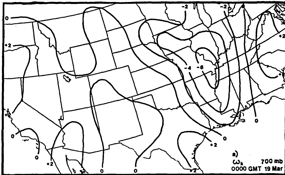
Fig. 9 As in Fig. 6, but for 0000 GMT 19 March 1986.
