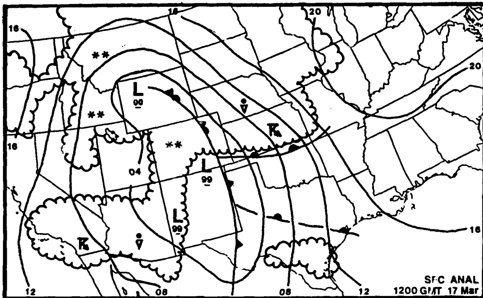
Fig. 2 Surface and 500 mb analyses for 1200 GMT 17 March 1986. At the surface, scalloped areas denote low and middle cloud ceilings that are either broken or overcast. At 500 mb, solid lines are height contours in decameters while dashed lines are isotherms in °C.
