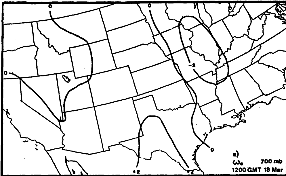
Fig. 13 As in Fig. 11, but for 1200 GMT 18 March 1986.
