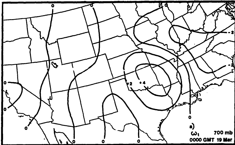
Fig. 22 As in Fig. 19, but for 0000 GMT 19 March 1986.
