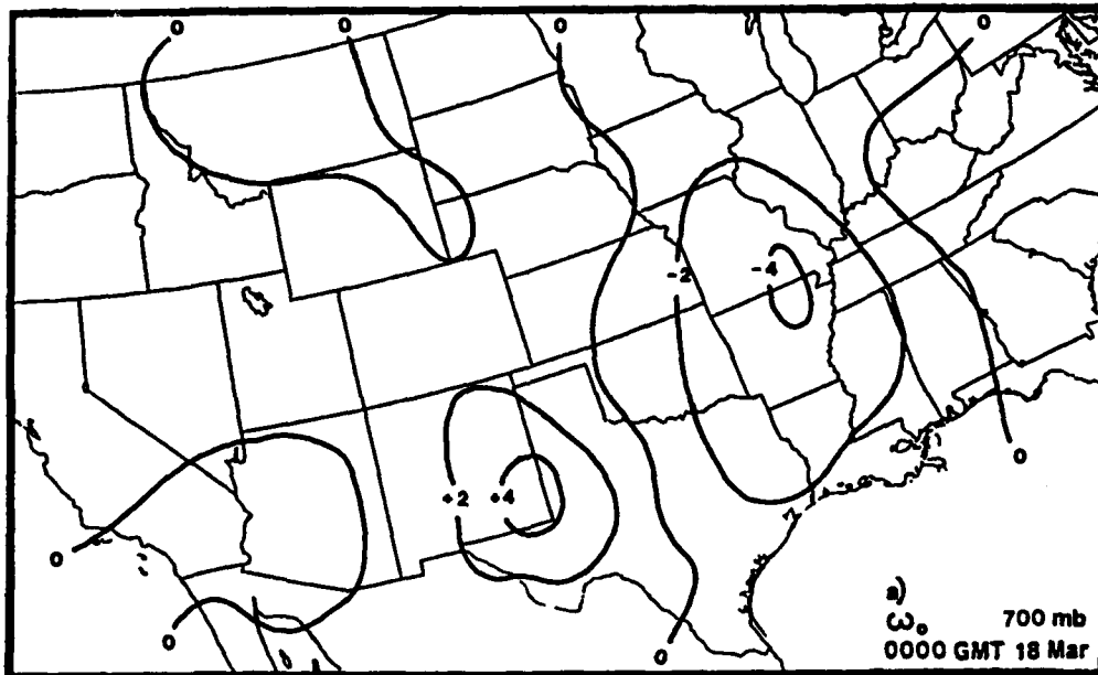
Fig. 12 As in Fig. 11, but for 0000 GMT 18 March 1986.
