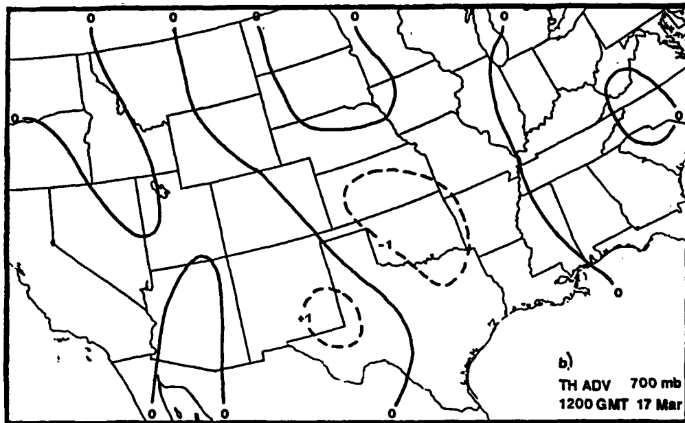
Fig. 15 Components of traditional omega equation vertical motion (microbars/s) at 700 mb on 1200 GMT 17 March 1986 due to a) differential vorticity advection and b) the horizontal Laplacian of thickness advection.
