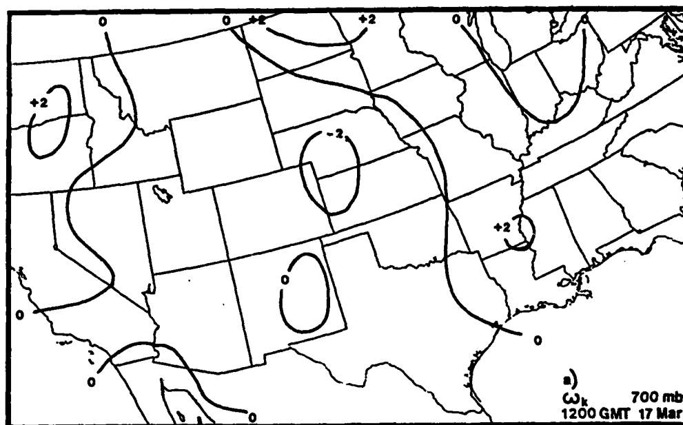
Fig. 6 Kinematic vertical motions (microbars/s) at a) 700 mb and b) 500 mb for 1200 GMT 17 March 1986.
