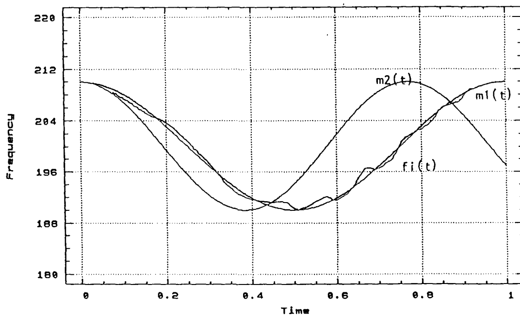
Fig. 4.4 Average Instantaneous Frequency Deviation for Tone Messages
