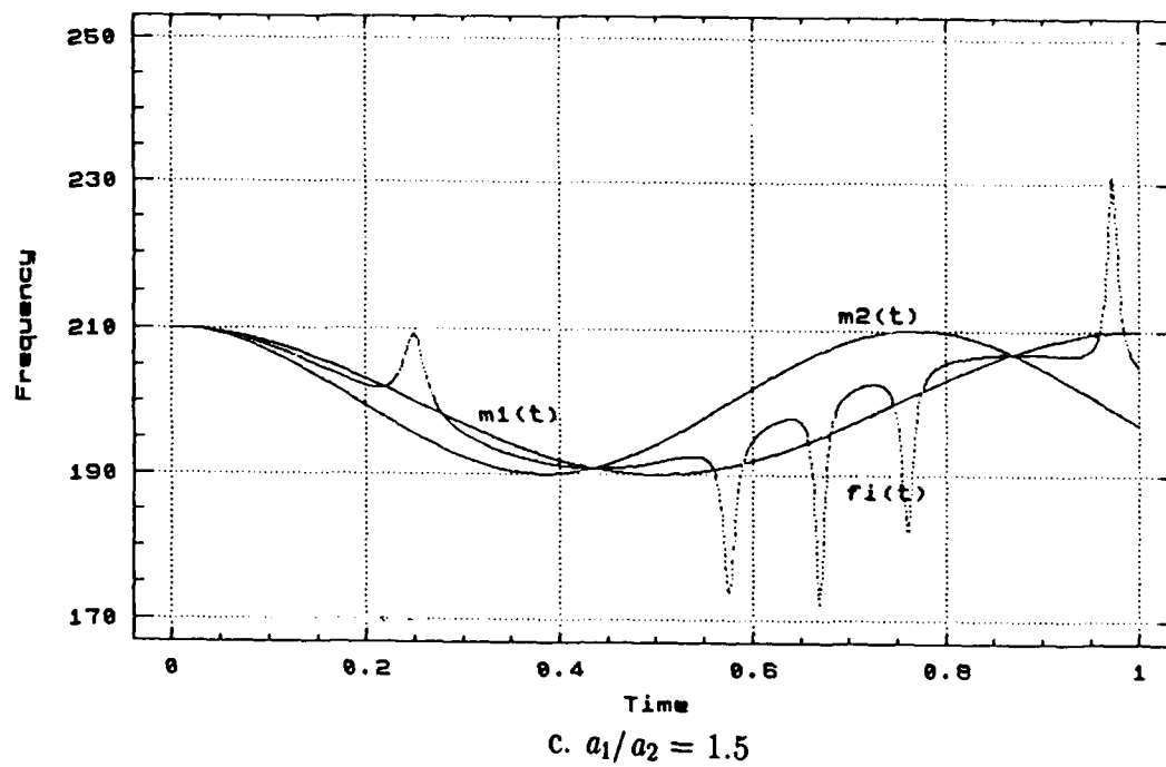
Fig. 2.2 Instantaneous Frequency for Tone Messages
