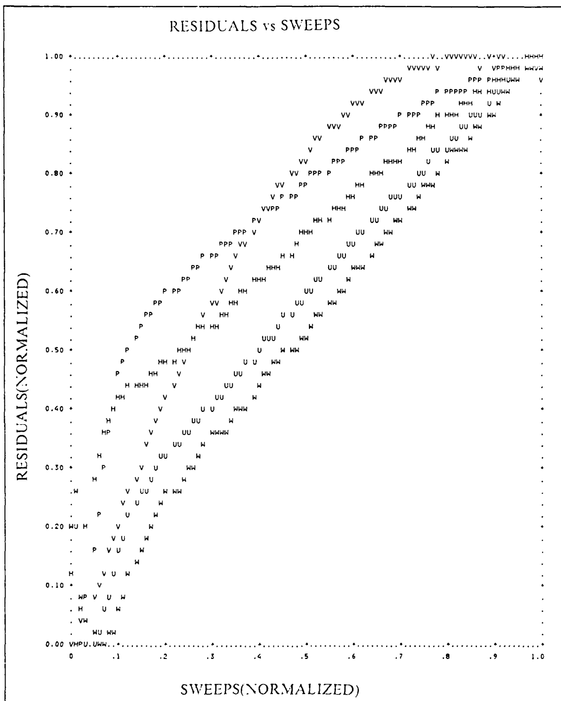
Figure 11. Sample Output Residuals vs Sweeps (Diverging Solution)
