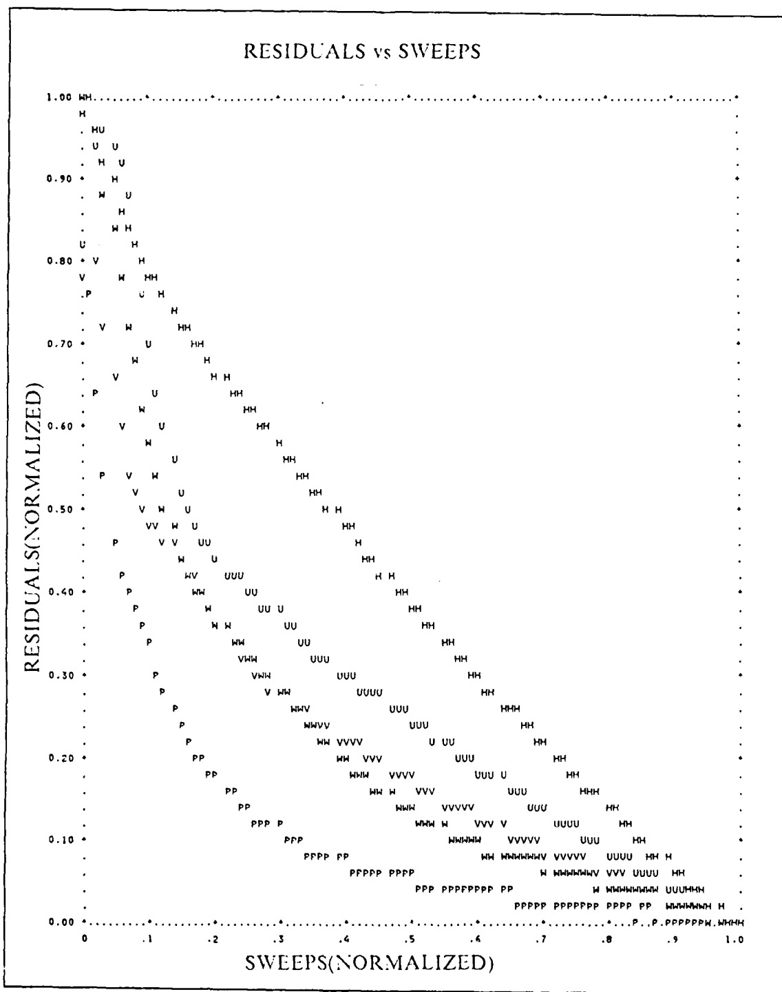
Figure 9. Sample Output Residuals vs Sweeps (Converging Solution)
