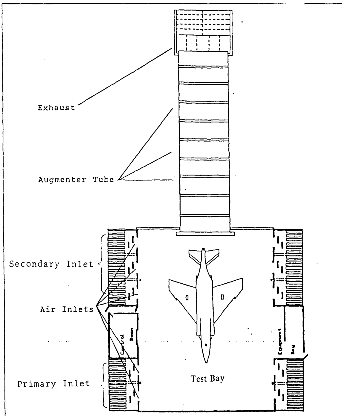
Figure 1. Actual Hush House (Top View Looking Down)
