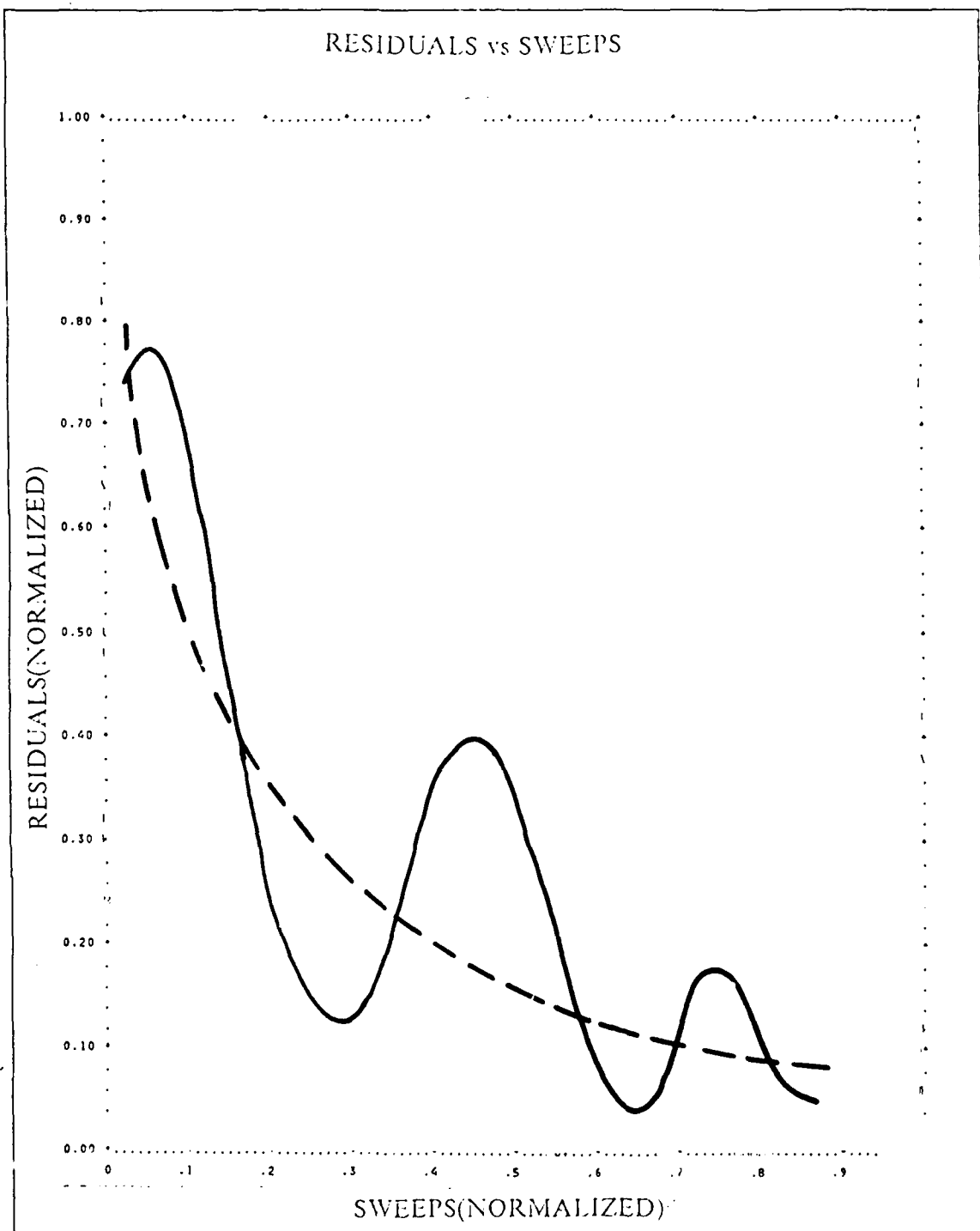
Figure 10. Sample Output Residuals vs Sweep (Converging Solution)
