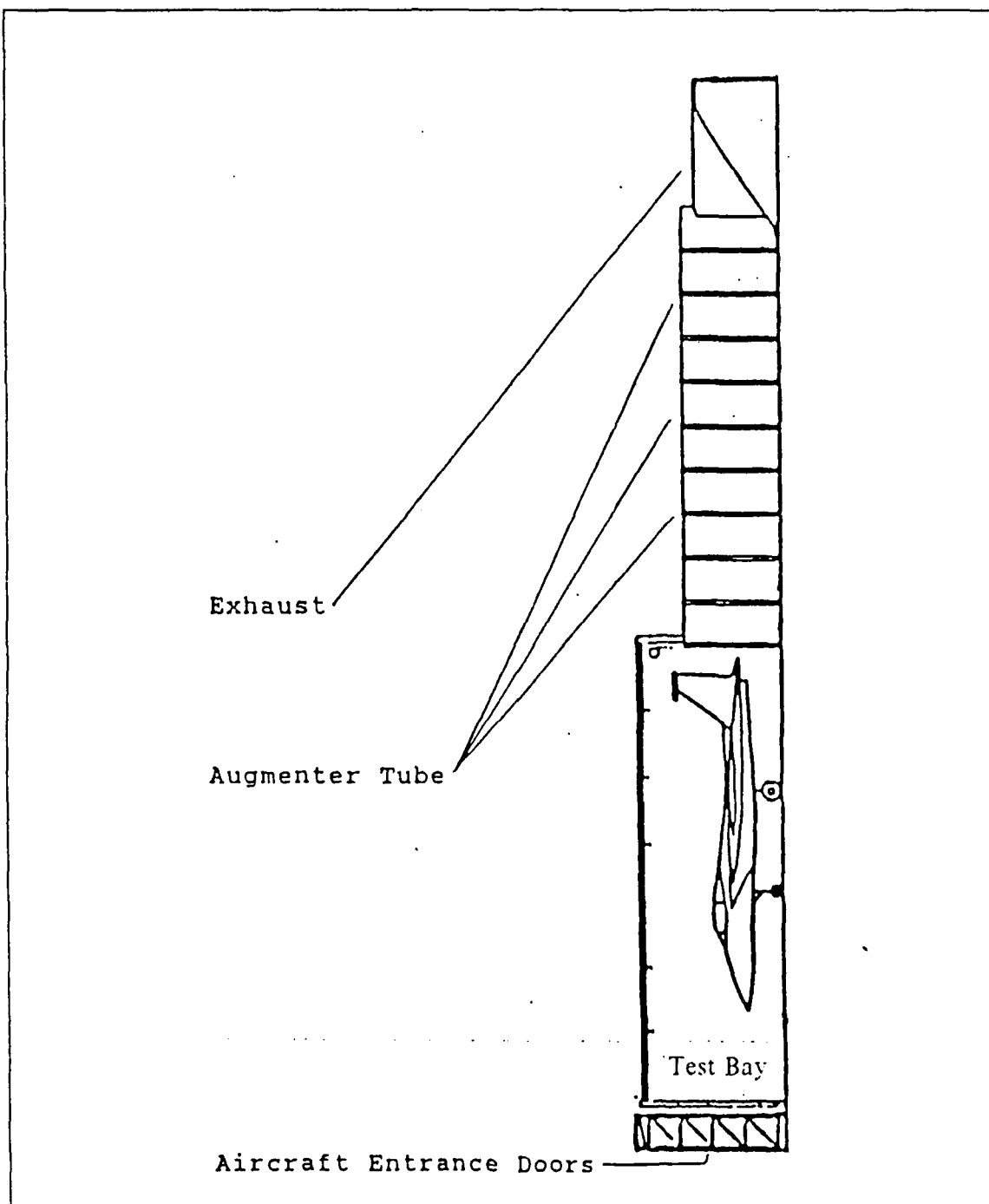
Figure 2. Actual Hush House (Side View)
