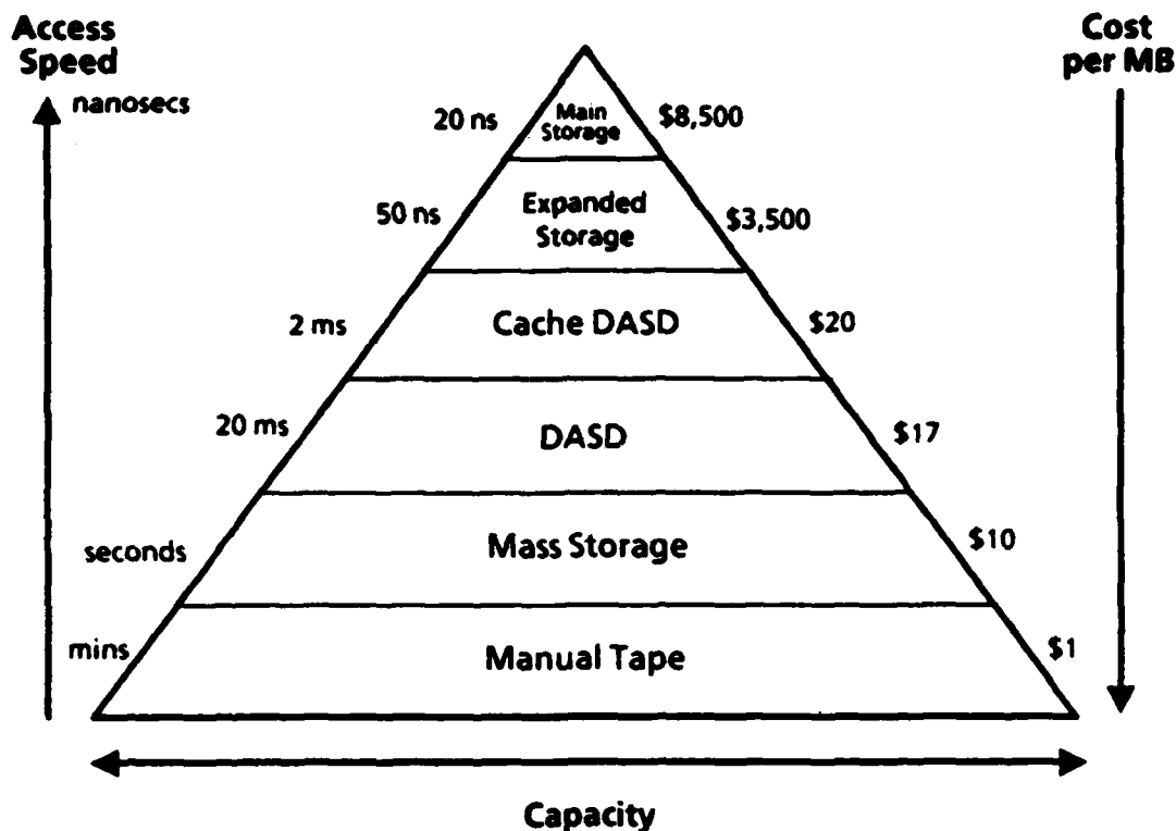
Figure 1. Information Storage Hierarchy
