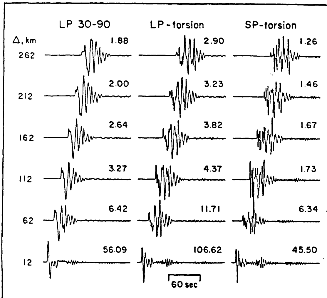
Figure 7. Comparison of the profile of Green's functions corresponding to a pure strike-slip source as recorded on the three instruments displayed earlier in Figure 1. Amplitudes are given in mm for a moment of 4\pi\rho \times 10^{25} dyne-cm.
