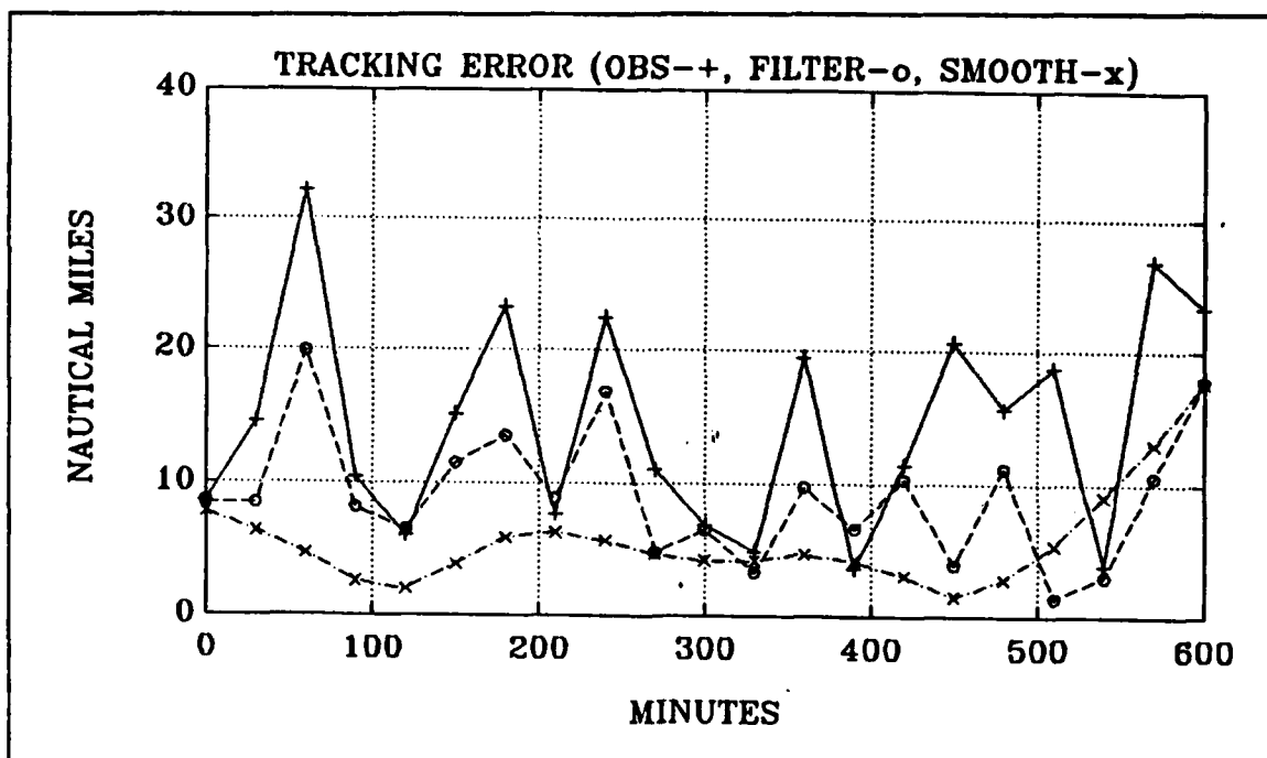
Figure 26. Position Error
