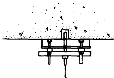
SIDE VIEW: SENSOR MOUNTING SYSTEM
