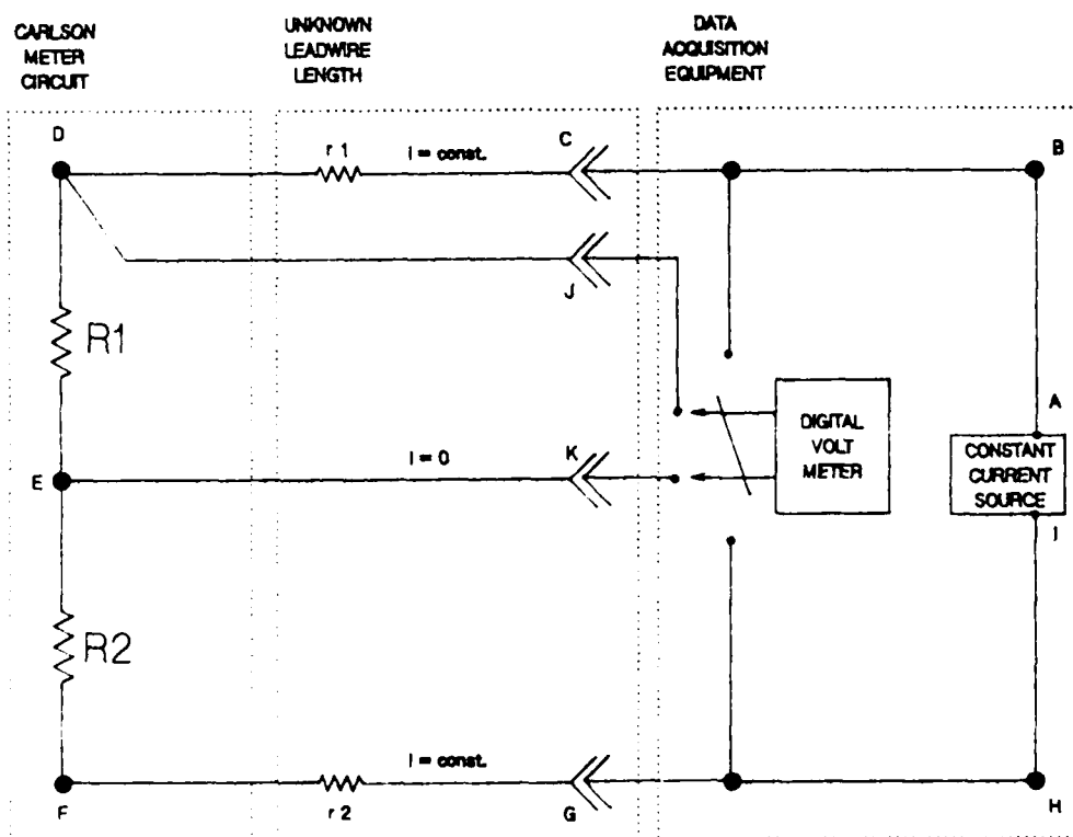
Figure 15. Carlson meter four-wire measurement circuit
