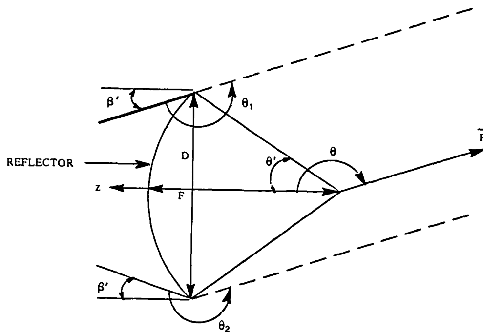
Figure 20. Geometry for Stationary Phase Evaluation of the Nonuniform Current Field
