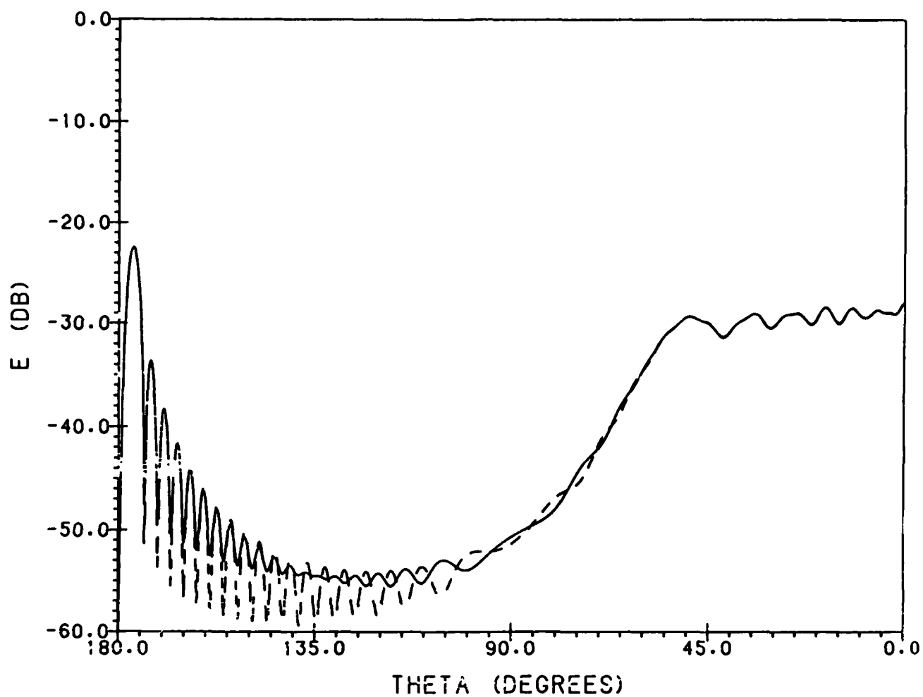
Figure 14c. \phi = 45^\circ Cross-Polar Amplitude Pattern of 20\lambda Dipole-Feed Paraboloid Antenna, Primary Field Not Included; - - - - PO, ——— PO + Nonuniform Current Field, F/D = 0.4 , \theta = [180^\circ, 0^\circ]
