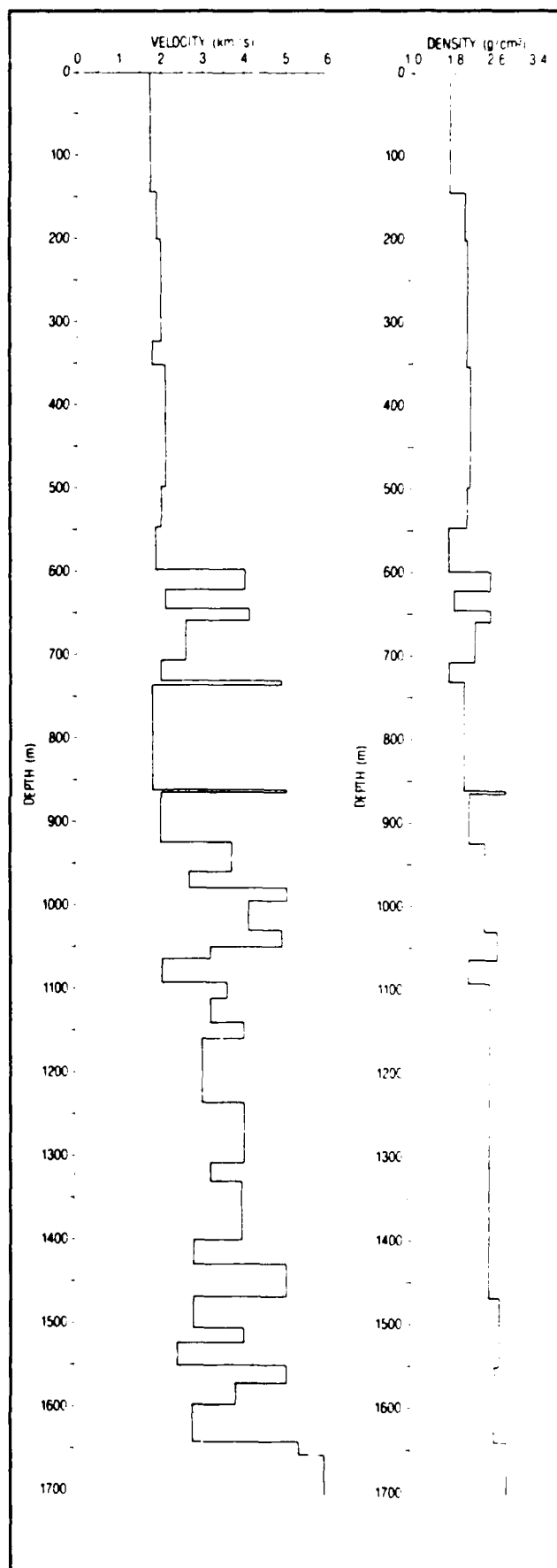
Figure 27 (right). Velocity and density as functions of depth for the proposed geoaoustic model presented in Figure 26.
