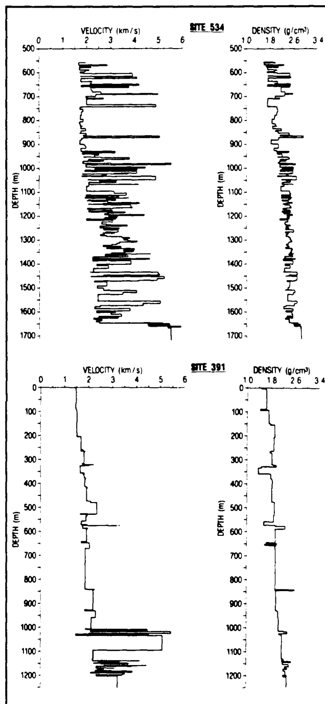
Figure 9. Velocity and density as functions of depth for DSDP sites 534 and 391. The data used to make these plots (Appendix A-1) are shipboard laboratory measurements of velocities and densities for samples at the given depths in the cores. No correction has been made for sediment rebound and no consideration has been given to sediment not recovered in the cores. The recovery rate for hole 534 was 56% and for hole 391 was 50.1%.
