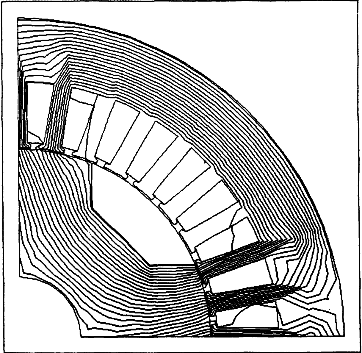
FIGURE 3.3.3.6. PEAK TORQUE POSITION WITH SUPERCONDUCTING MATERIAL ON ROTOR
