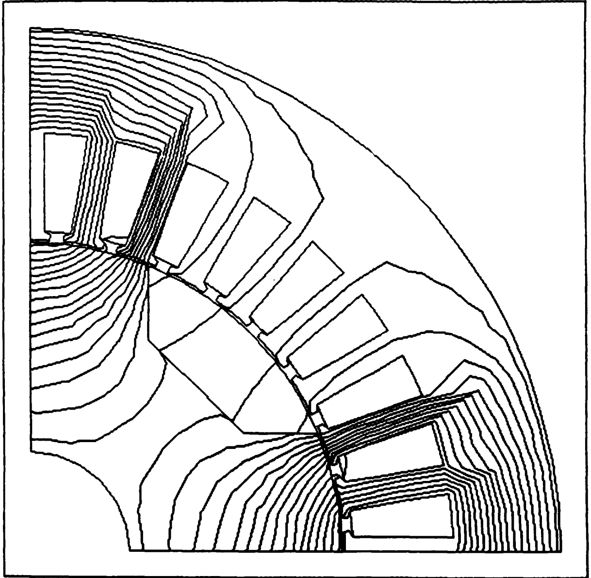
FIGURE 3.3.3.2. QUADRATURE AXIS FLUX WITH CONVENTIONAL ROTOR
