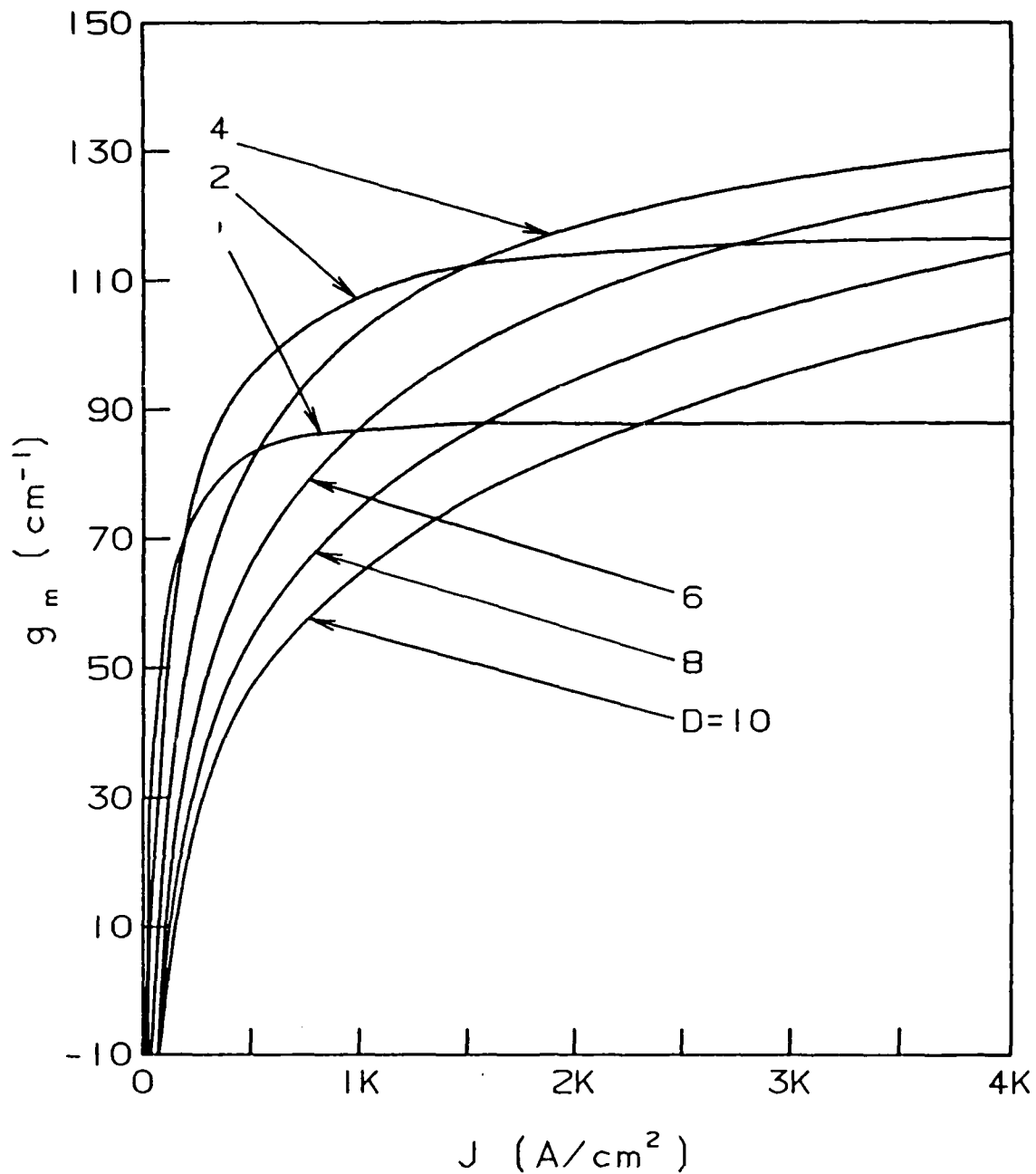
Fig. 9 Computed mode gain versus current density for a single quantum well with the electron density of states equal to that of a regular single-quantum well, while the hole density of states is D times that of the electron density of states.
