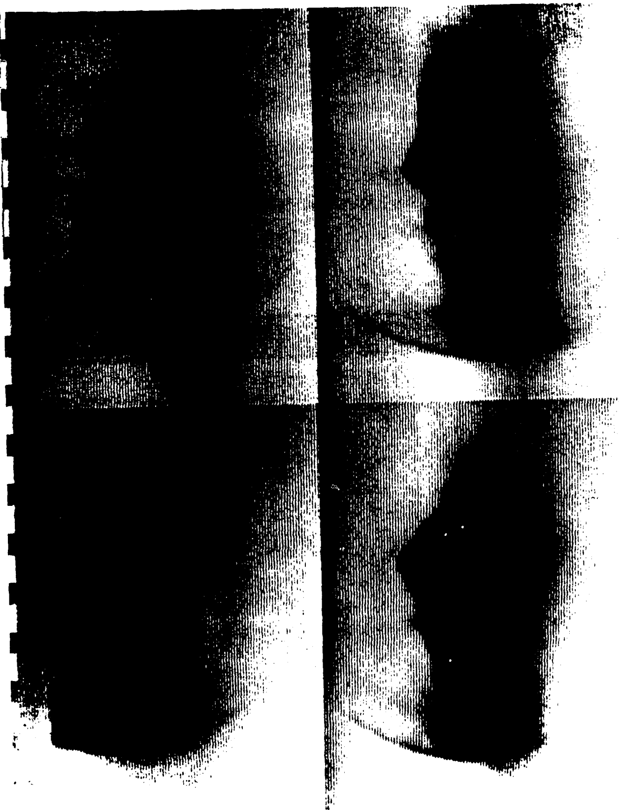
Figure 8. Time resolved black-and-white photos show flow structures similar to those envisioned by two-dimensional hydrocodes. Note the Mach disc indicating underexpanded flow from the plasmajet source and the concave nose of the propagating jet (seen also in the calculated images).
