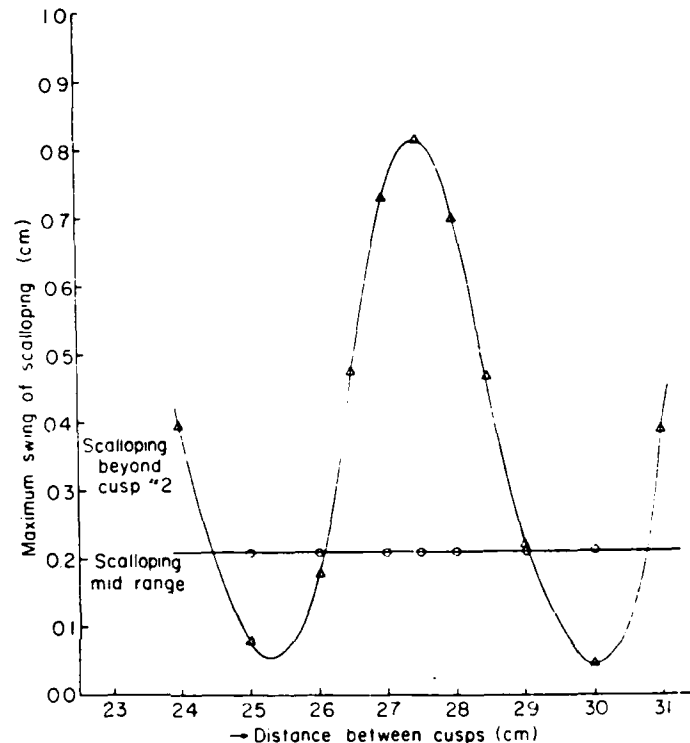
Figure 7. The range of scalloping, as defined by the difference between the maximum and minimum radii of the trajectories in the region between the cusps and beyond the second cusp. Shown is the case of variations due to distance between cusps, B_0 = 328.8 gauss, r_{\text{start}} = 1.5 cm, V_0 = 26 kV, and \zeta_{1,2} = 4 mm.
