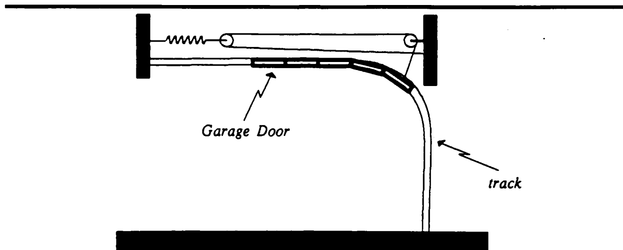
Figure 10.1: Sliding garage door in open, equilibrium position.
