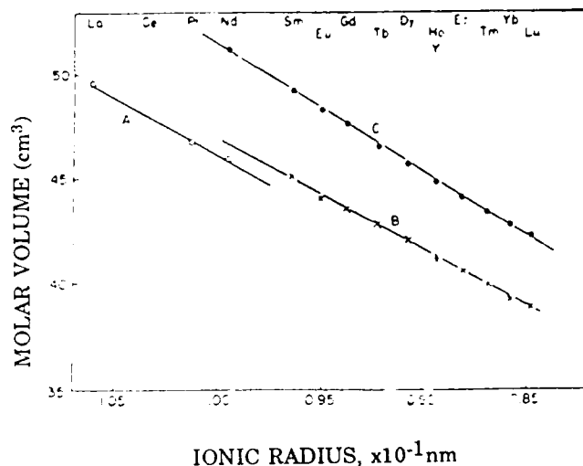
Fig. 4. Molecular volumes of the A, B, and C crystal structures in the lanthanide sesquioxides. 48
