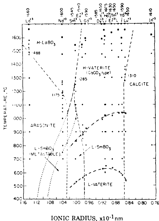
Fig. 12. Stability relations of the \text{ABO}_3 -type borates as a function of temperature and ionic radius of the large cation. 145
