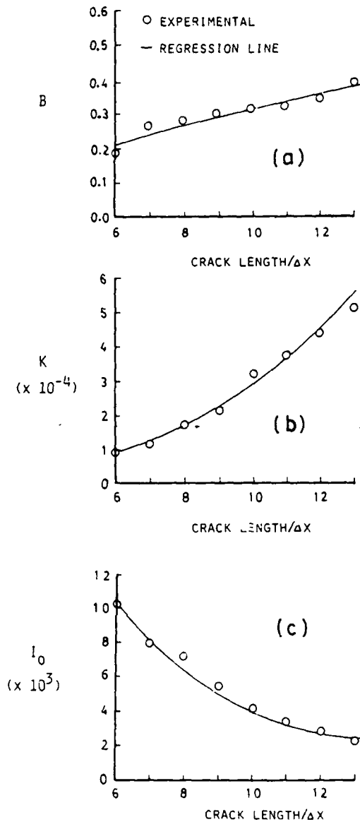
Fig. 8. Relationship between B , K and I_0 and crack length position for Test Condition I for Ref. [16].
