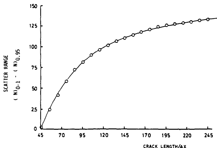
Fig. 14. Variation of scatter range as function of crack length position.
