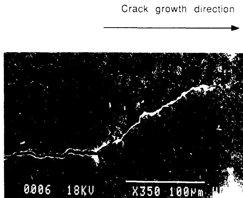
Figure 14(a) Change in the crack orientation due to overload
