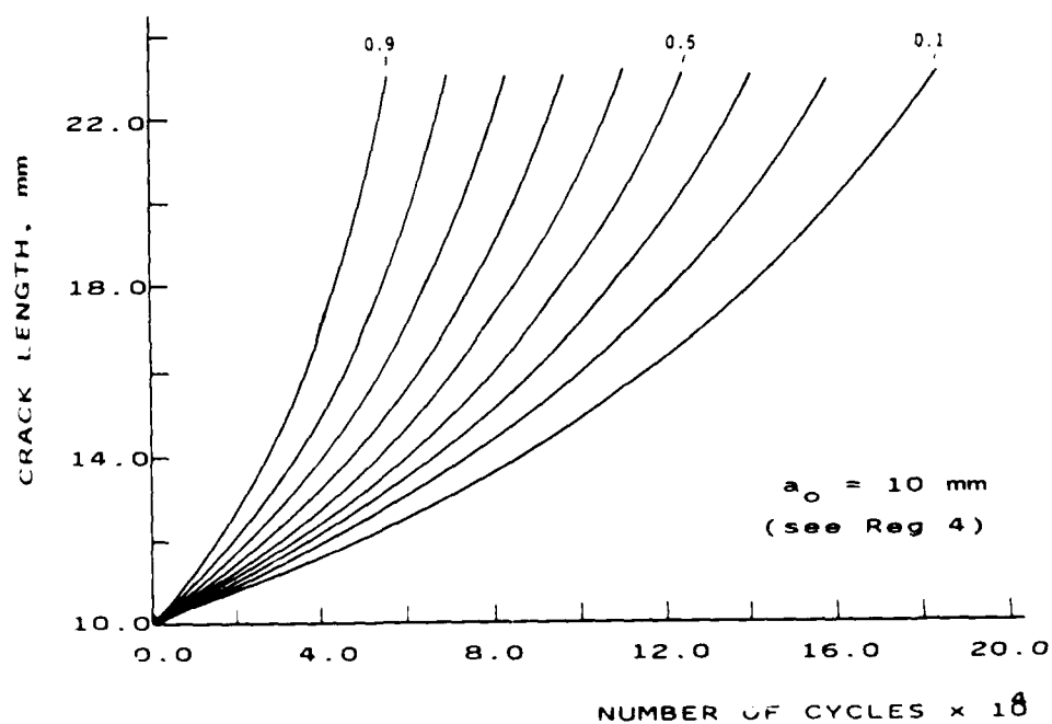
Fig. 7(b). Constant-probability curves generated from data in Fig. 7(a).
