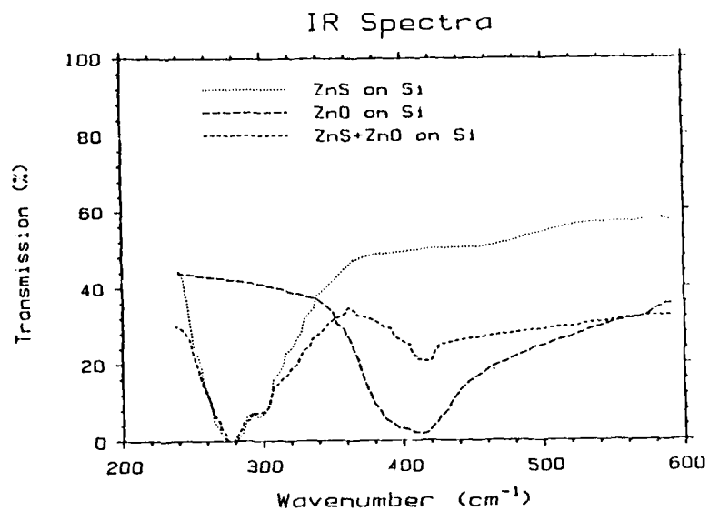
Fig. 3. Comparative infrared spectra of films of untreated zinc oxide, zinc oxide partially converted to the sulfide, and of fully converted zinc sulfide.
