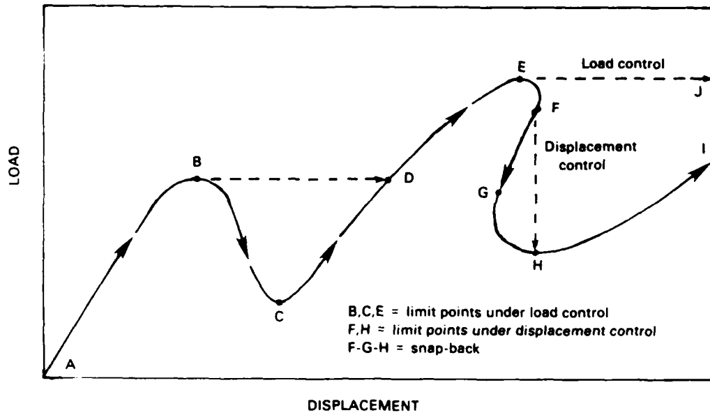
Figure 9. Snap-back phenomenon.
