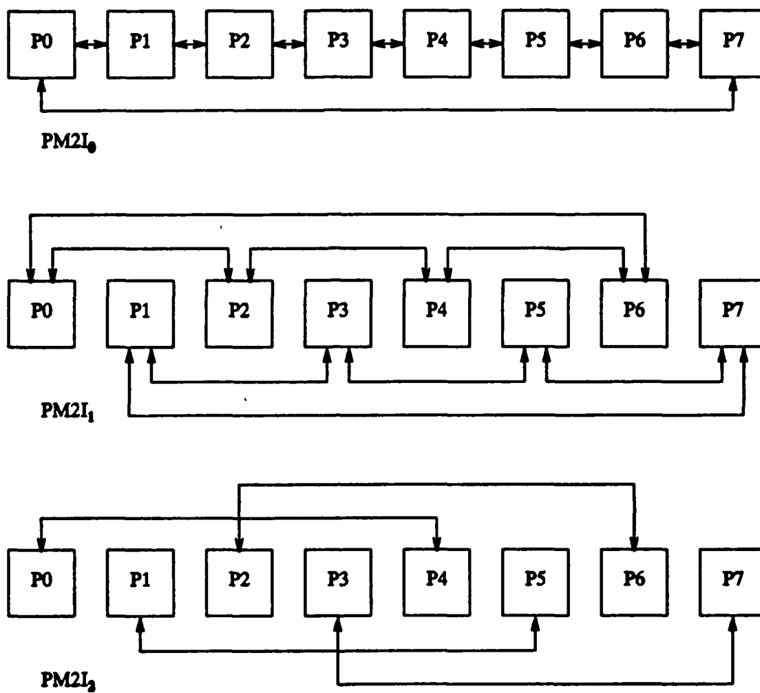
Figure 1.2.12. PM2I network for N=8 .
