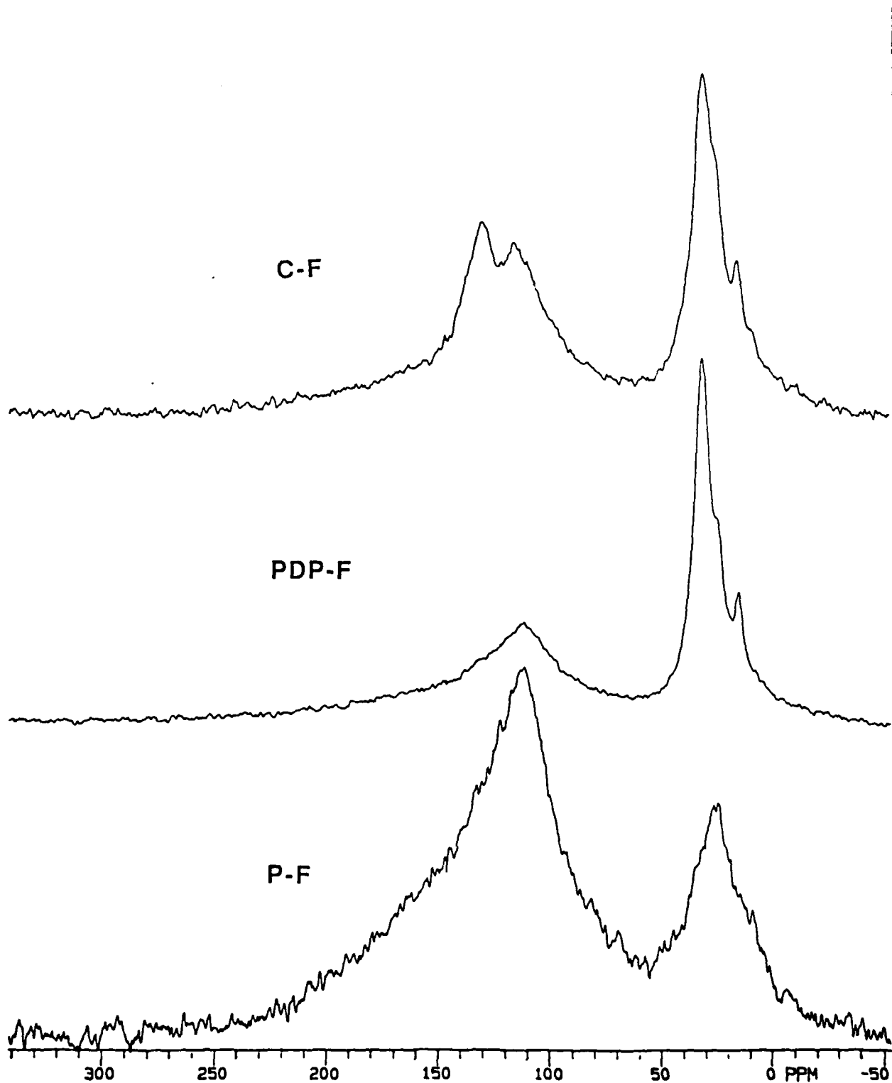
Fig. 1. Liquid like ^{13}\text{C} spectra of phenol-formaldehyde (P-F), 3-n-pentadecylphenol-formaldehyde (PDP-F) and cashew-formaldehyde (C-F).
