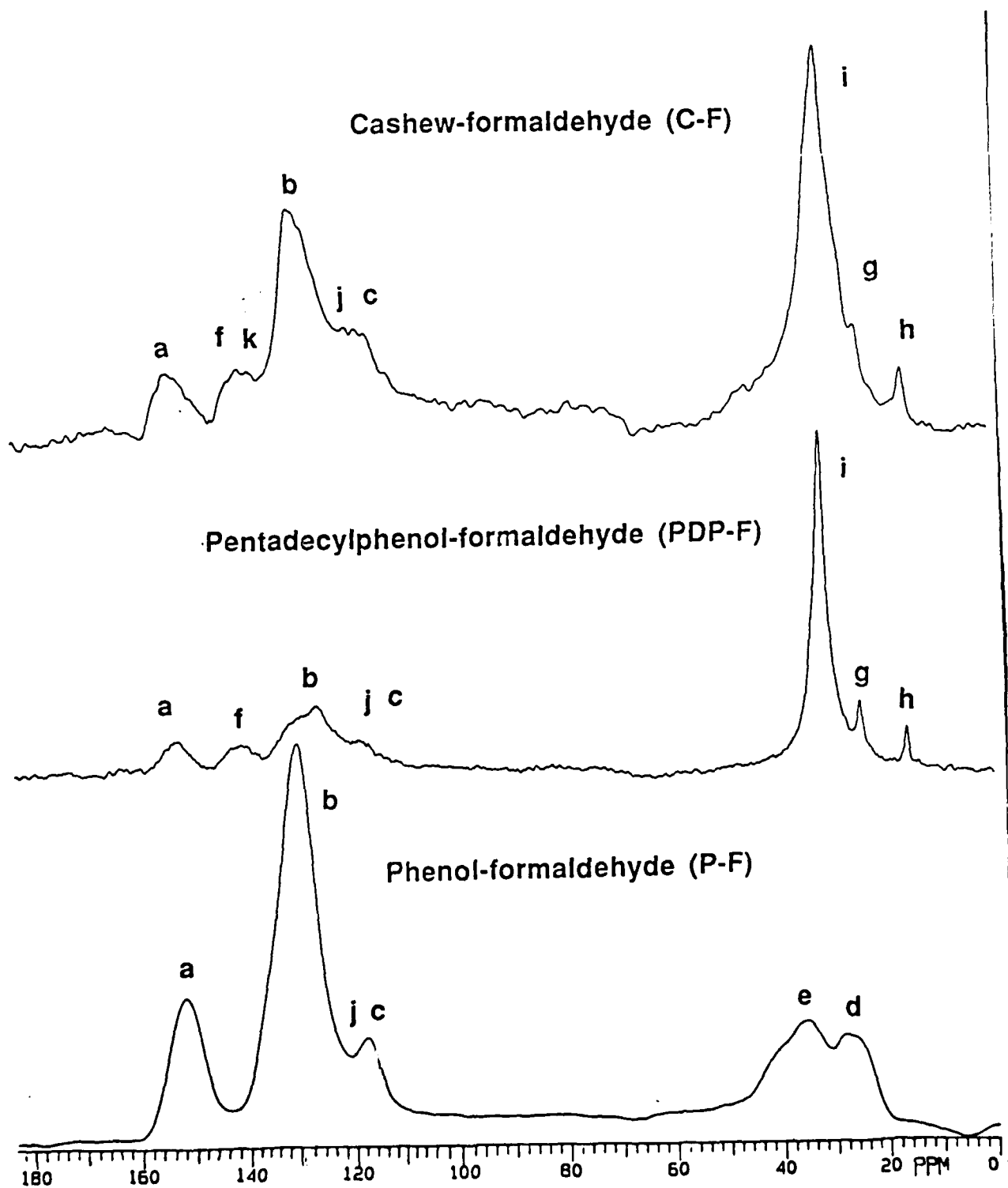
Fig. 2. Solid-state ^{13}\text{C} -NMR spectra of phenol-formaldehyde (P-F), 3-n-pentadecylphenol-formaldehyde (PDP-F) and cashew-formaldehyde (C-F) using CP/MAS/DD and TOSS.
