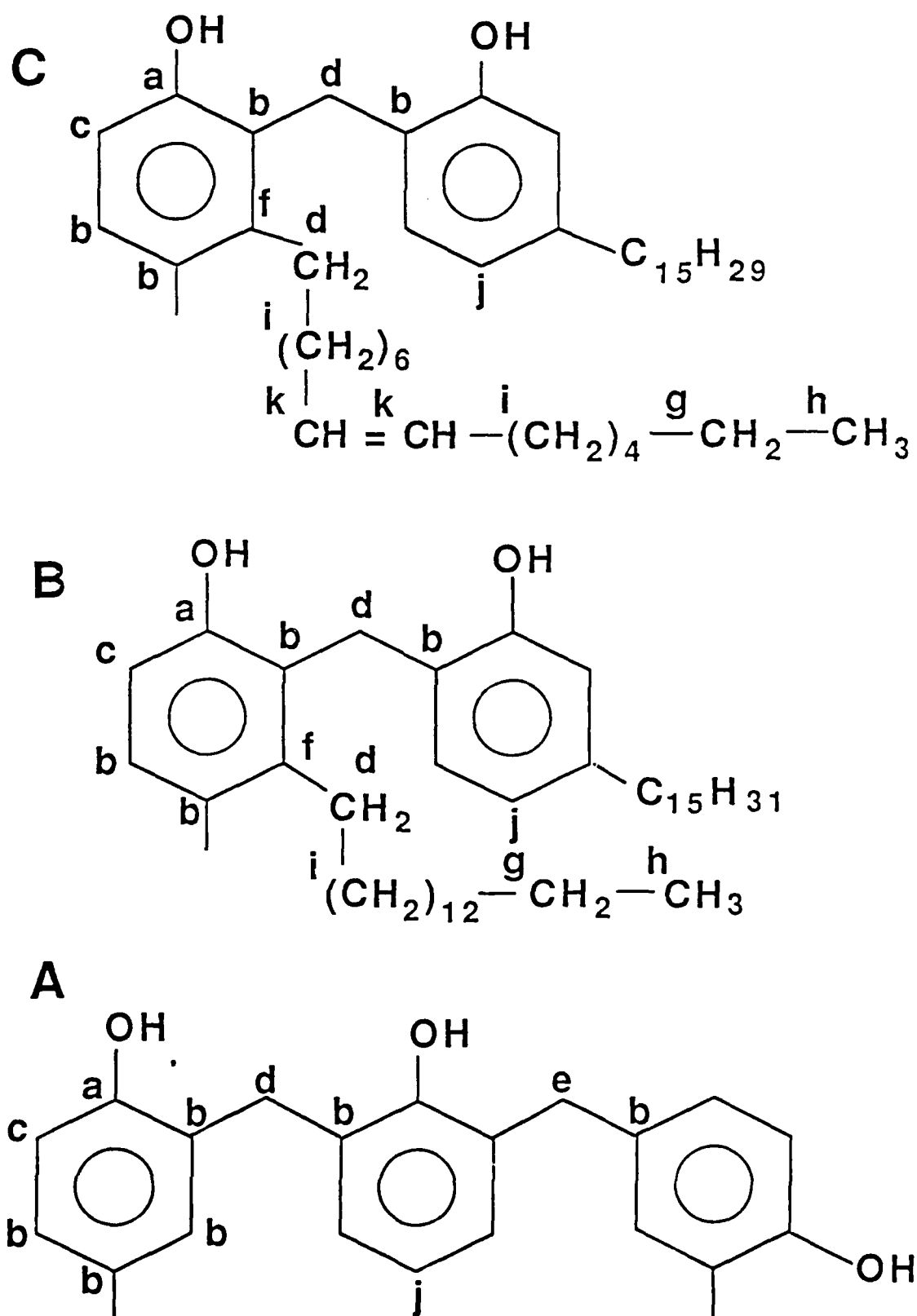
Fig. 3. Structural assignments of solid-state ^{13}\text{C} -NMR spectra. The letter designations used here are used to assign the spectra in Figure 2. The structures shown are the simplest representation of the crosslinked resin for (A) phenol-formaldehyde (P-F), (B) 3-n-pentadecylphenol-formaldehyde (PDP-F) and (C) cashew-formaldehyde (C-
