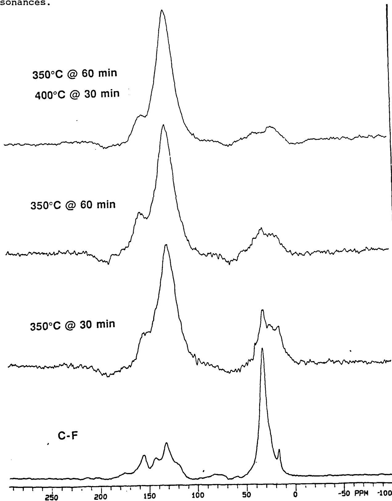
Fig. 5. Solid-state ^{13}\text{C} -NMR spectra using CP/MAS/DD and TOSS of cashew formaldehyde (C-F) thermally degraded at different temperature and time periods noted in the figure. Note that the chemical shift scale is different than the other spectra reflecting the broader resonances.
