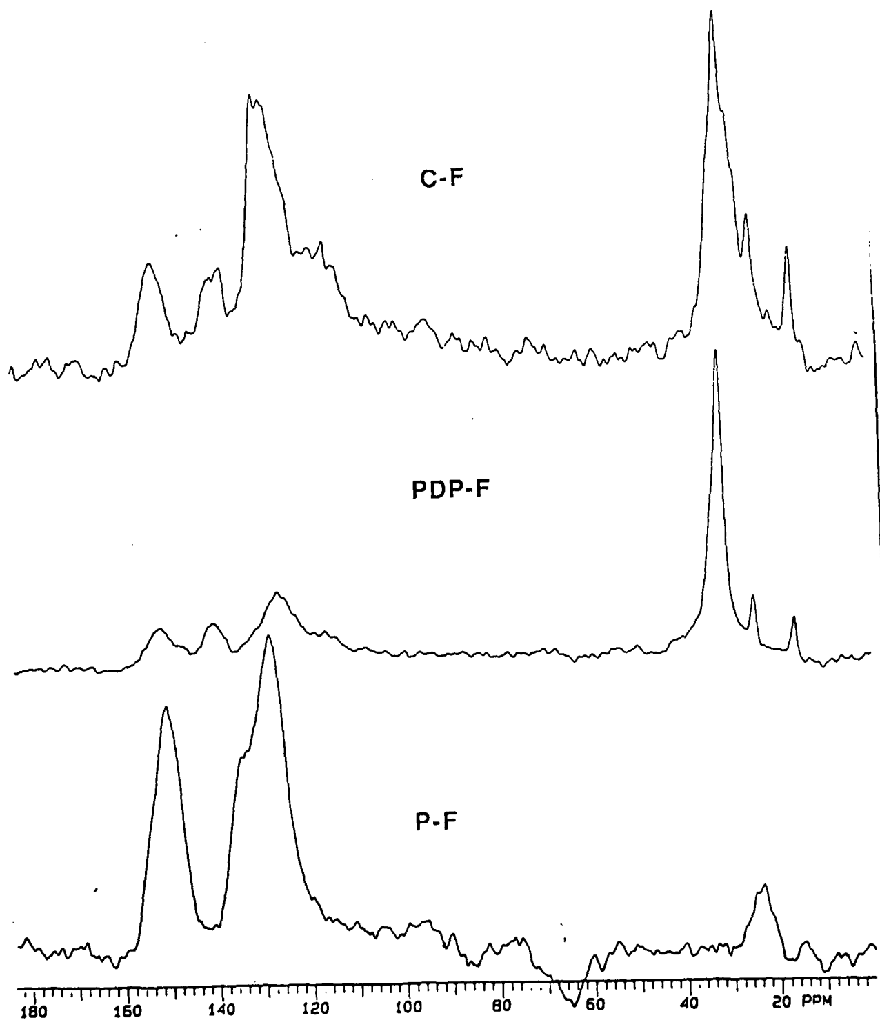
Fig. 4. Proton-dephased TOSS ^{13}\text{C} -NMR spectra of phenol-formaldehyde (P-F), 3-n-pentadecylphenol-formaldehyde (PDP-F) and cashew-formaldehyde (C-F). Incomplete spinning sideband elimination is evident between 50 and 90 ppm.
