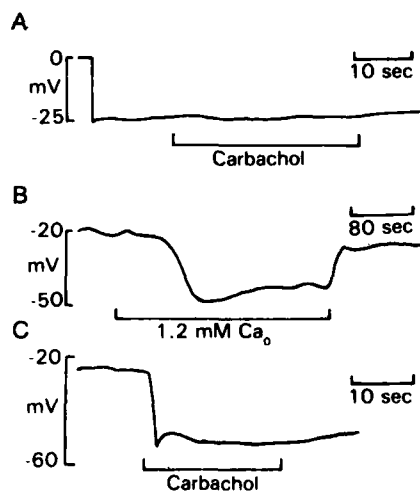
FIG. 2. Voltage responses of Me_2BAPTA -loaded cell stimulated in zero- Ca^{2+} medium. A Me_2BAPTA -loaded cell was impaled (rapid deflection at beginning of trace) in zero- Ca^{2+} medium. The cell was exposed to 1 mM carbachol (A and C) or 1.2 mM Ca^{2+} (B) as indicated. The traces in A–C are a continuous record. As observed by others (4), exposure to Ca^{2+} medium in the absence of carbachol (B) caused the membrane to hyperpolarize; the ionic basis for this effect is unknown. It was not associated with a fura-2-detectable rise in [Ca^{2+}]_i (data not shown).
