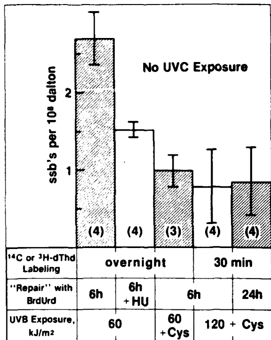
Figure 2. UVB-photolytic breakage of radiolabeled LY-R DNA: the effects of labeling the opposite strand with BrdUrd; the effects of HU presence during repair or Cys during photolysis. The mean number of ssb's was calculated as described in Materials and Methods; the number of experiments performed is shown in parentheses. As indicated in the figure, cells were radiolabeled either for thirty minutes or overnight. LY-R and LY-S cells behaved identically under these conditions.
