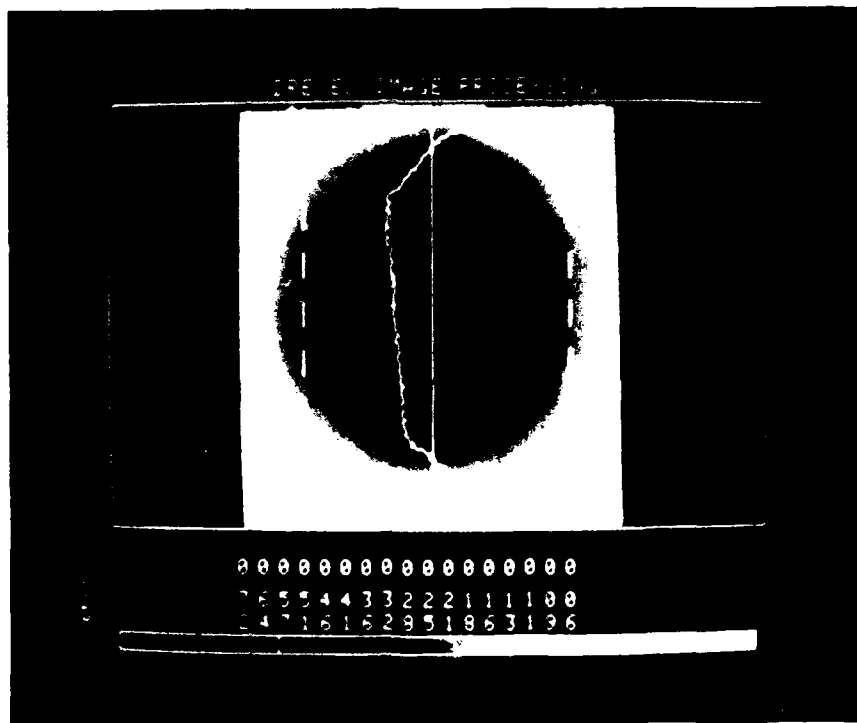
Fig. 10. Beam uniformity and penumbra analysis in the vertical axis. Due to the 35° angle of the x-ray tube during irradiation the optical density is greater close to the tube and less as the distance increases, relative to the center of the beam. The dose rate across the useful area of the beam varies by approximately ± 5%.
