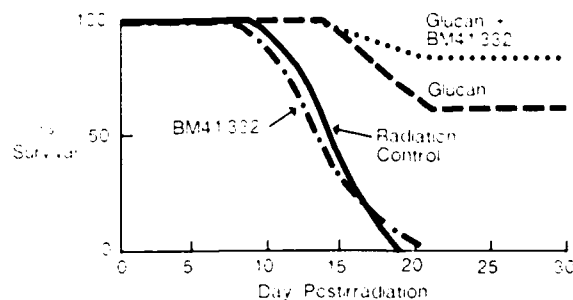
FIG. 4 Effects of combined BM41.332 and glucan administration on survival of irradiated C3H/HeN mice. Approximately 20 hr prior to 9.0 Gy ^{60}\text{Co} radiation, mice were injected i.v. with particulate glucan (75 mg/kg), BM41.332 (10 mg/kg), or both substances. Data represent cumulative survival data obtained from 47–77 mice in each treatment group.
