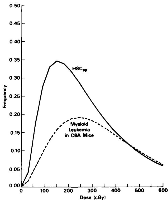
Fig. 4 Relative marrow concentration of HSC PR plotted as a function of dose 2 d postirradiation. —, curve generated by the equation (1 - e^{-D/0.6 \text{ Gy}})^{1.93} = (1 - e^{-D/2.2 \text{ Gy}})^{1.03} (see text for explanation); ---, curve generated by the equation 2.4 \times 10^{-5} D^2 e^{-8.25 \times 10^{-3} D} , which predicts the frequency of myeloid leukemia as a function of dose in postirradiated CBA male mice. The D_0 and n values for CFU-S IM were determined to be 0.95 Gy and 1.02.
