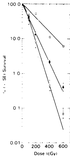
Fig. 3 Dose-response curves for CFU-S. ●—●, CFU-S IM measured immediately postirradiation; ○—○, CFU-S 2d measured 2 d postirradiation; □—□, HSCs measured by flow cytometry 2 d postirradiation. One hundred thousand cells were measured by flow cytometry per point.
