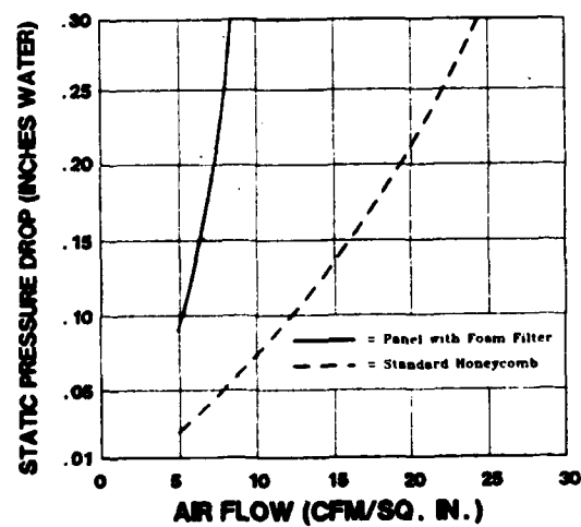
Figure 2-15. Air flow characteristics of a honeycomb panel.
