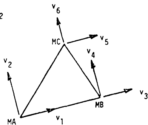
(b) Triangular Membrane Element
