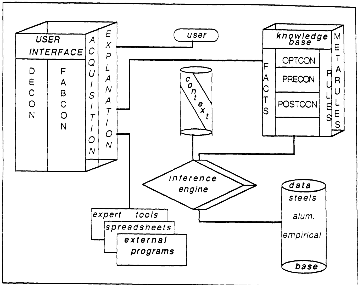
Figure 6.11: DISCON Architecture
