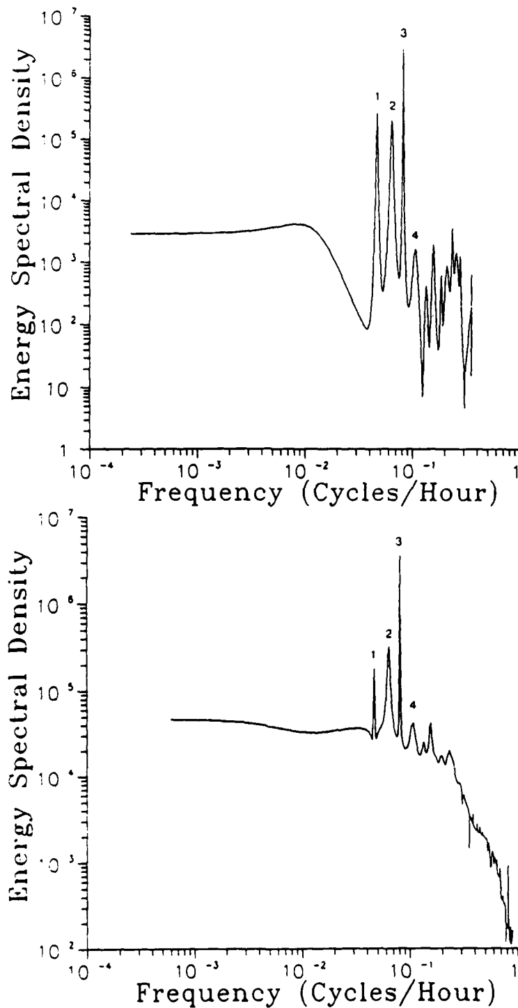
Figure 2.10: Prony's method estimates of the energy spectral density (cycles 2 /cph 2 ) of the detrended phase series (Figure 2.7).
