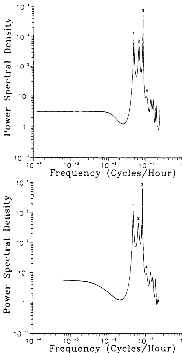
Figure 2.9: Autoregressive method estimates of the power spectral density (cycles 2 /cph) of the detrended phase series (Figure 2.7).
