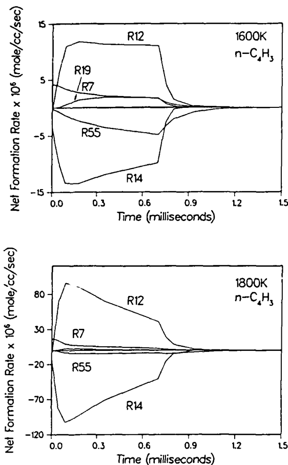
FIG. 2. Net Formation Rate for Production/Deconstruction of the n\text{-C}_4\text{H}_3 Radical. 2a) at 1600K, 2b) at 1800K.
