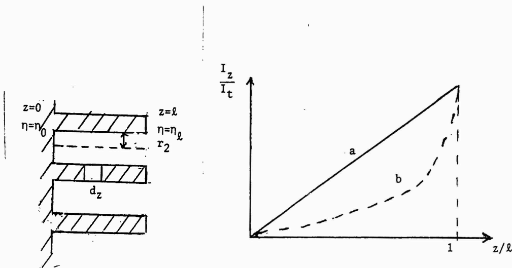
Fig. 5: The straight pore model for diffusion electrodes and the current distribution.
