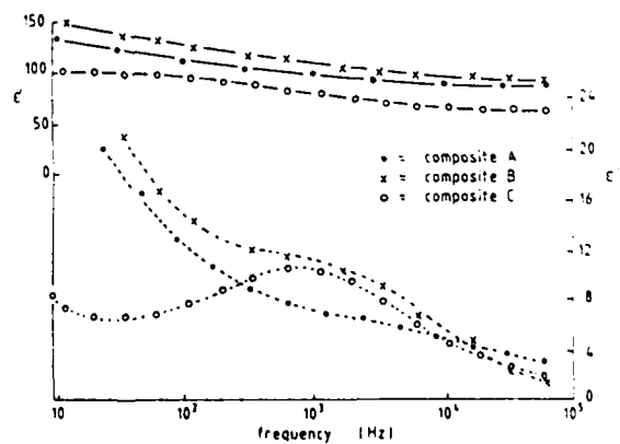
Figure 2: The behaviour of \epsilon' and \epsilon'' against frequency in ceramic/polymer composites at 363 K. \epsilon' = —, \epsilon'' = - - -
