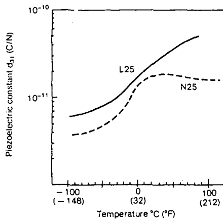
Figure 1 Piezoelectric Constant vs. Temperature
