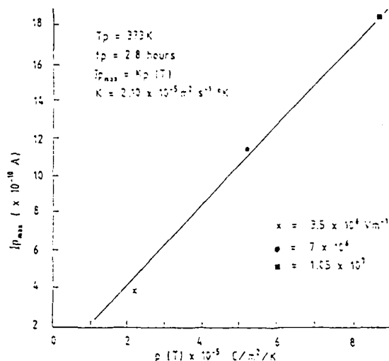
Fig. 5: Peak current against pyroelectric coefficient at 333 K in PZT5/PVDF (A) (50/50).
