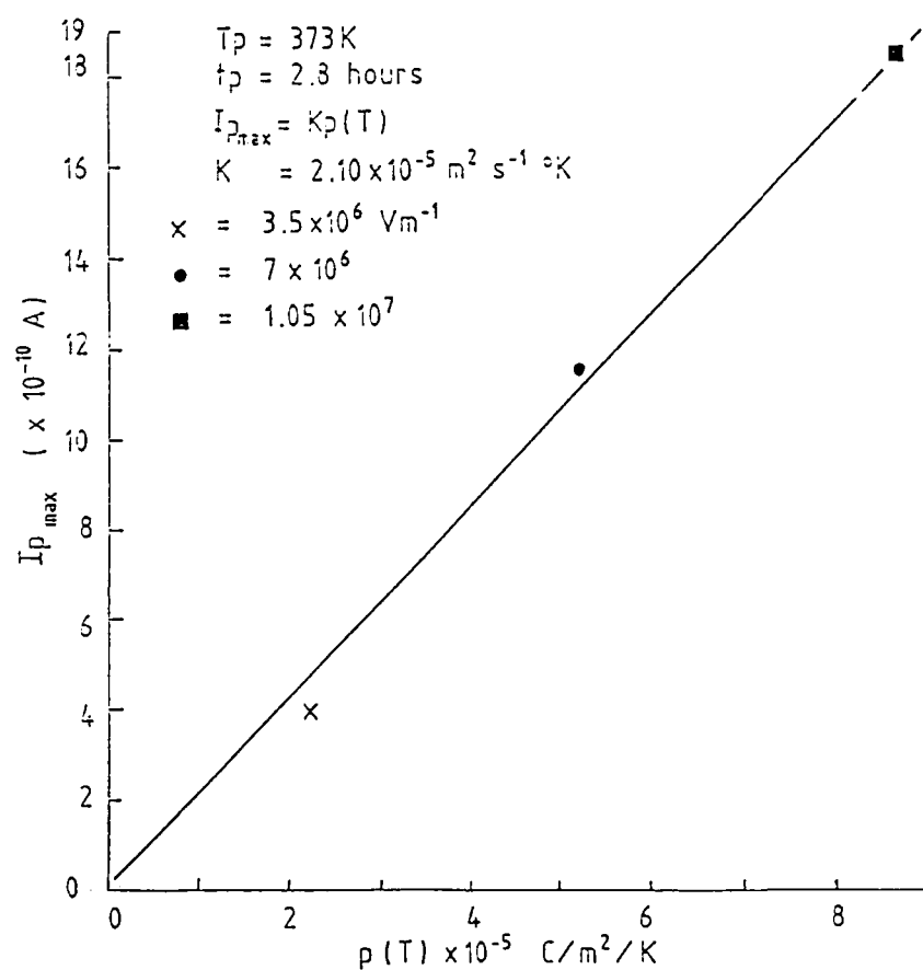
Fig. 10 : Peak current against pyroelectric coefficient at 333K in PZT5 / VDF-TrFE (Composite C)
