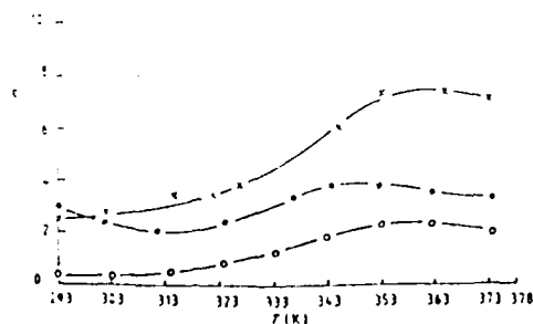
Figure 6 Dielectric loss behaviour against temperature in PZT/PVDF and piezel at 1 kHz. (x) PZT (50 vol% PVDF), (o) piezel, (triangle) PZT (10 vol% PVDF).
