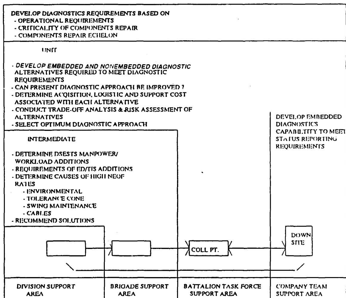
FIGURE 9. Integrated Diagnostic Methodology
