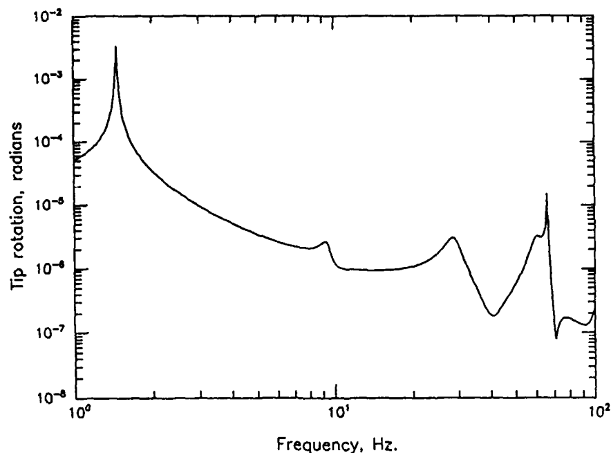
Figure 19. Truss with active controllers: initial response
