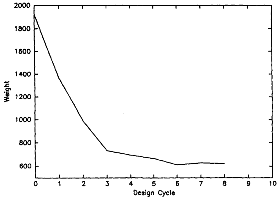
Figure 17. Truss transient weight history, alternate starting design
