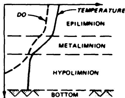
Figure 1. Cross section of a thermally stratified reservoir indicating location and characteristics of the epilimnion, metalimnion, and hypolimnion. Inset depicts typical temperature and dissolved oxygen profiles (from Keeley et al. 1978)
