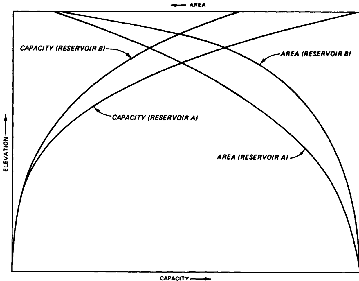
Figure 3. Area-capacity curves for two reservoirs having similar depth and surface area but differing volume and morphometry
