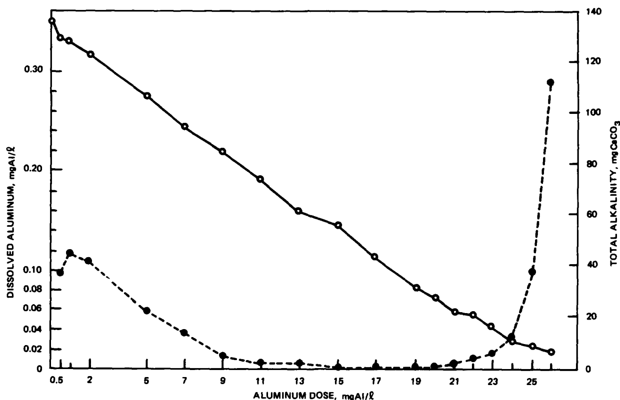
Figure 6. Changes in dissolved aluminum concentration (dashed line) and total alkalinity (solid line) for water from West Twin Lake, Ohio, treated with increasing doses of aluminum sulfate (after Cooke et al. 1978)
