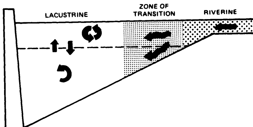
Figure 2. Schematic representation of longitudinal zonation in a typical reservoir. Arrows indicate dominant transport processes. Changes in shading indicate decline in turbidity from the riverine to lacustrine zones (after Thornton et al. 1980)
