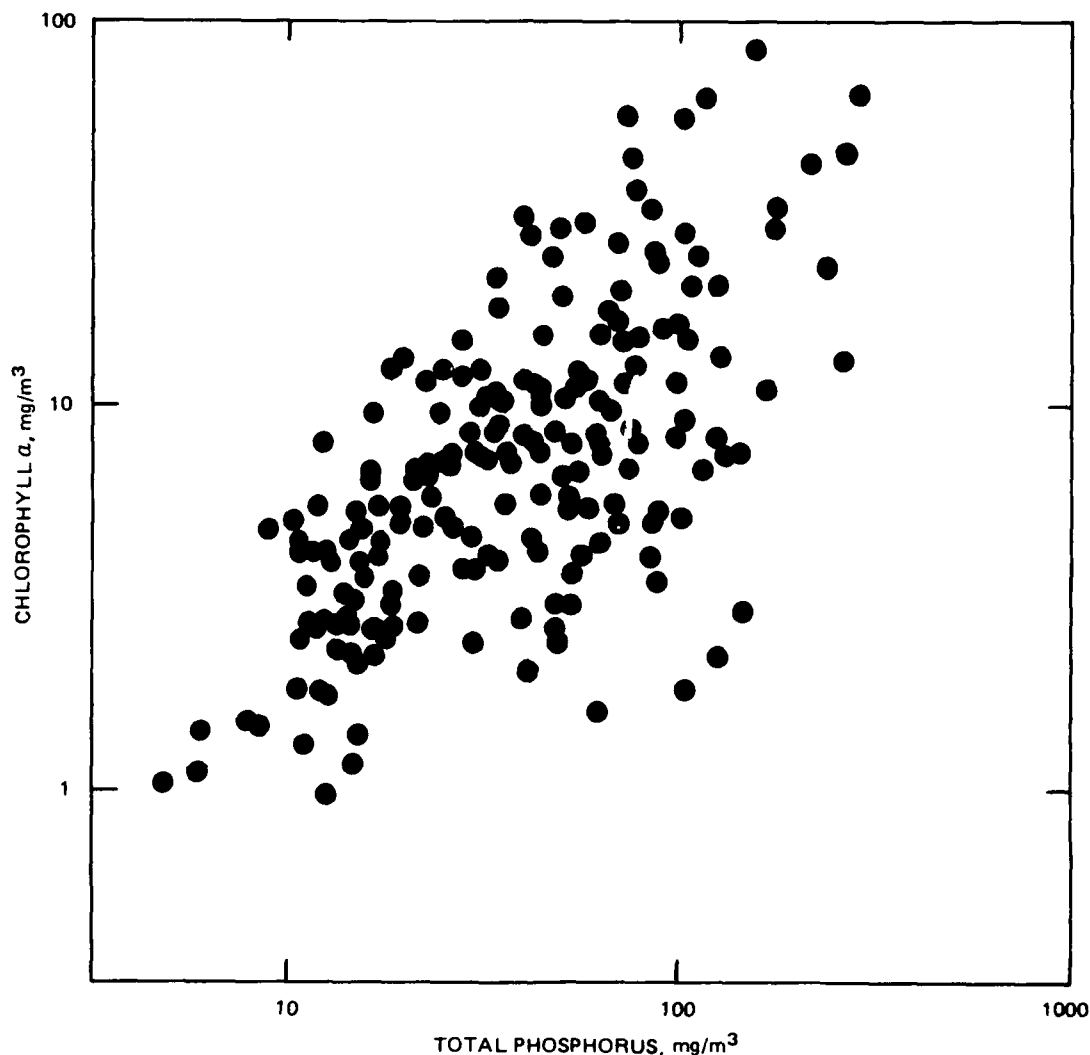
Figure 5. Relationship of average, growing-season chlorophyll a concentration and spring total phosphorus concentration for CE reservoirs (after from Walker 1982)
