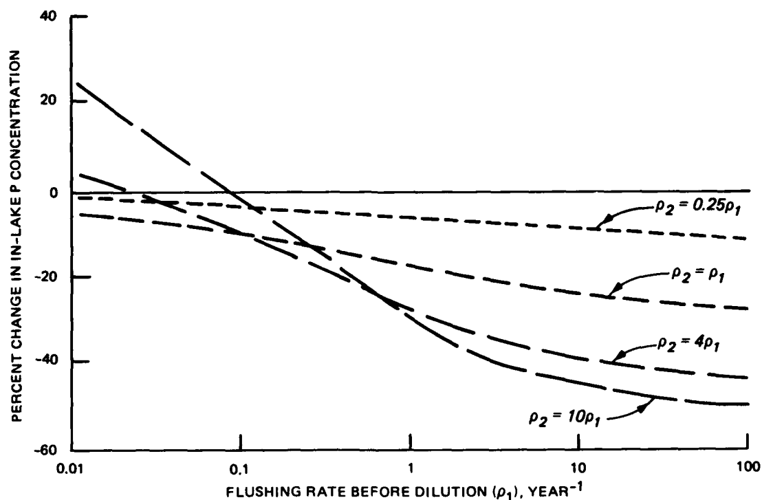
Figure 10. Percent change in in-lake phosphorus concentration following dilution with water having a phosphorus concentration that is 40 percent of the normal, undiluted inflow water (after Uttormark and Hutchins 1978). (See text for explanation)
