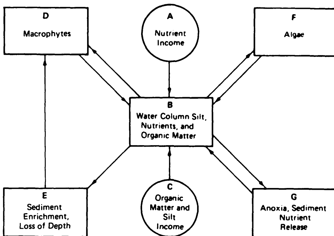
Figure 4. Primary interactions and effects of eutrophication in reservoirs and lakes (after Cooke et al. 1986)
