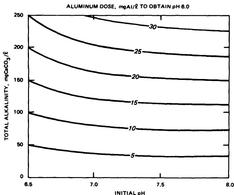
Figure 7. Estimated aluminum sulfate dose ( \text{mg Al } \ell^{-1} ) required to obtain pH 6 (i.e., "maximum dose") in treated water of varying initial alkalinity and pH (from Kennedy and Cooke 1982)
