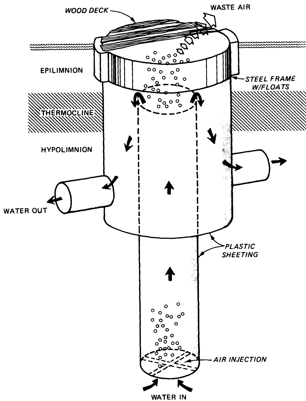
Figure 12. Example of a full air lift hypolimnetic aeration system (after Fast 1971)
