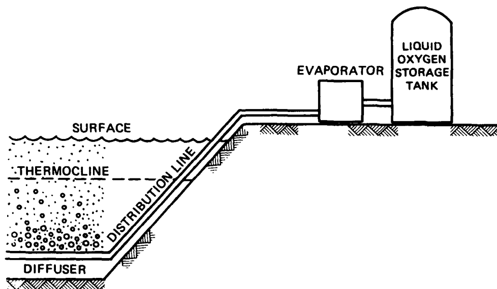
b. Generalized diagram
