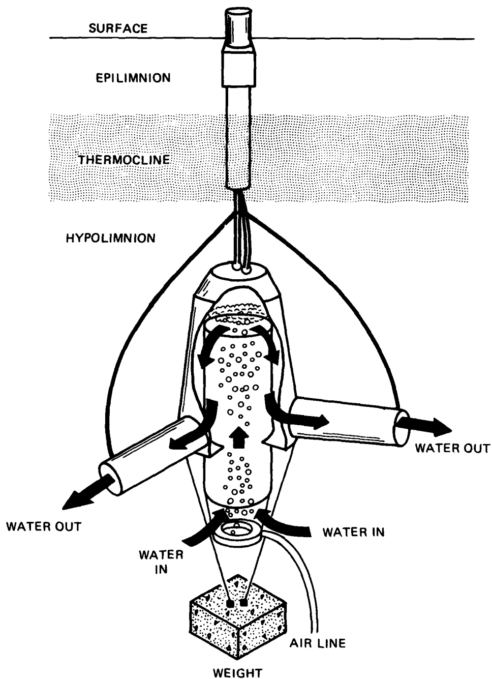
Figure 11. Example of a partial air lift hypolimnetic aeration system (after Fast 1975)
