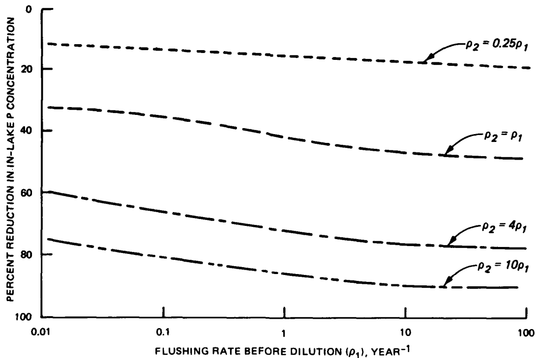
Figure 9. Percent change in in-lake phosphorus concentration following dilution with water containing no phosphorus (after Uttormark and Hutchins 1978). (See text for explanation)
