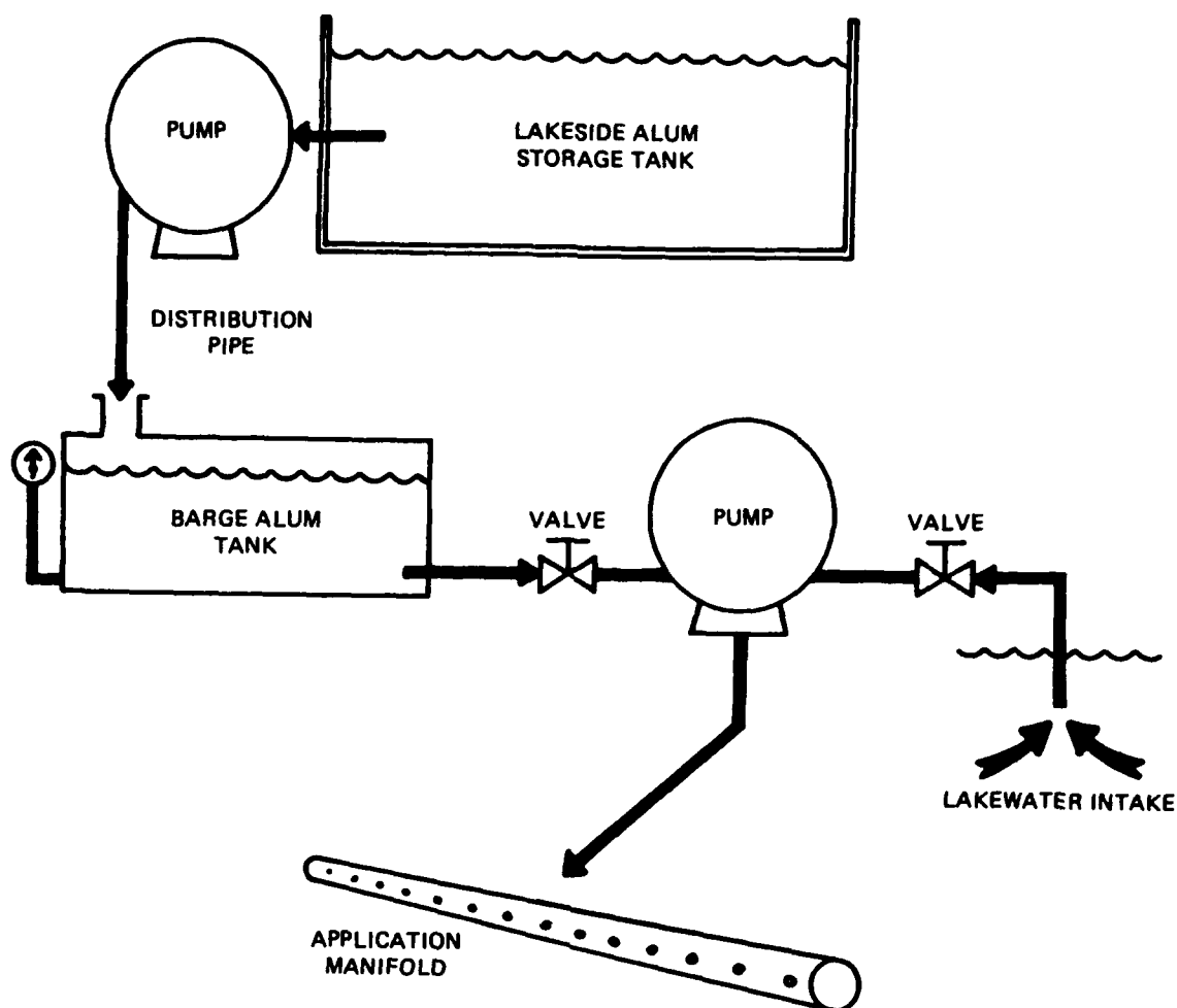
Figure 8. Generalized diagram of an alum application system (from Kennedy and Cooke 1982)
