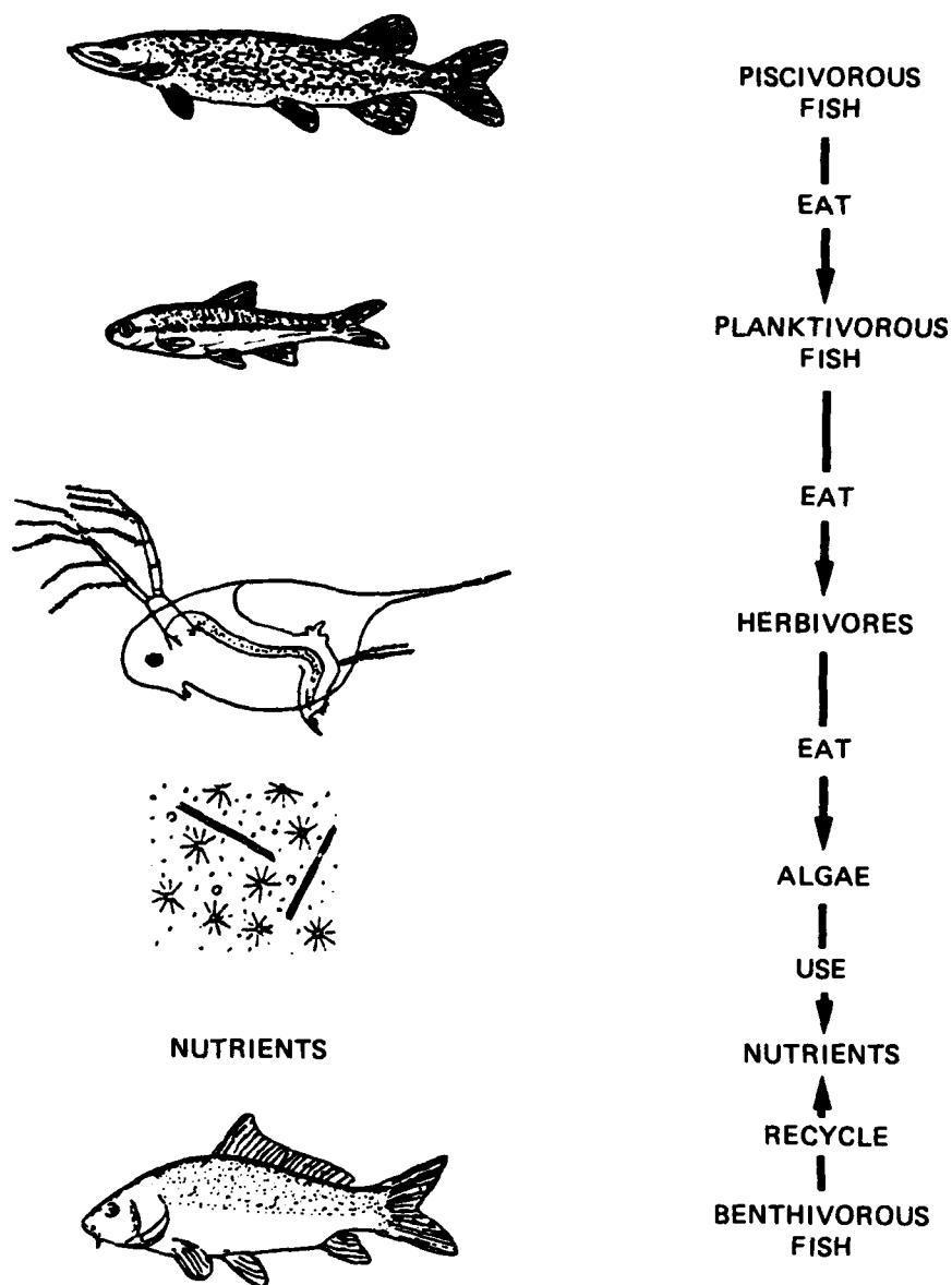
Figure 14. The aquatic food chain, indicating interactions between the components of the biomanipulation model (after Shapiro et al. 1982). See text for an explanation of the biomanipulation model
